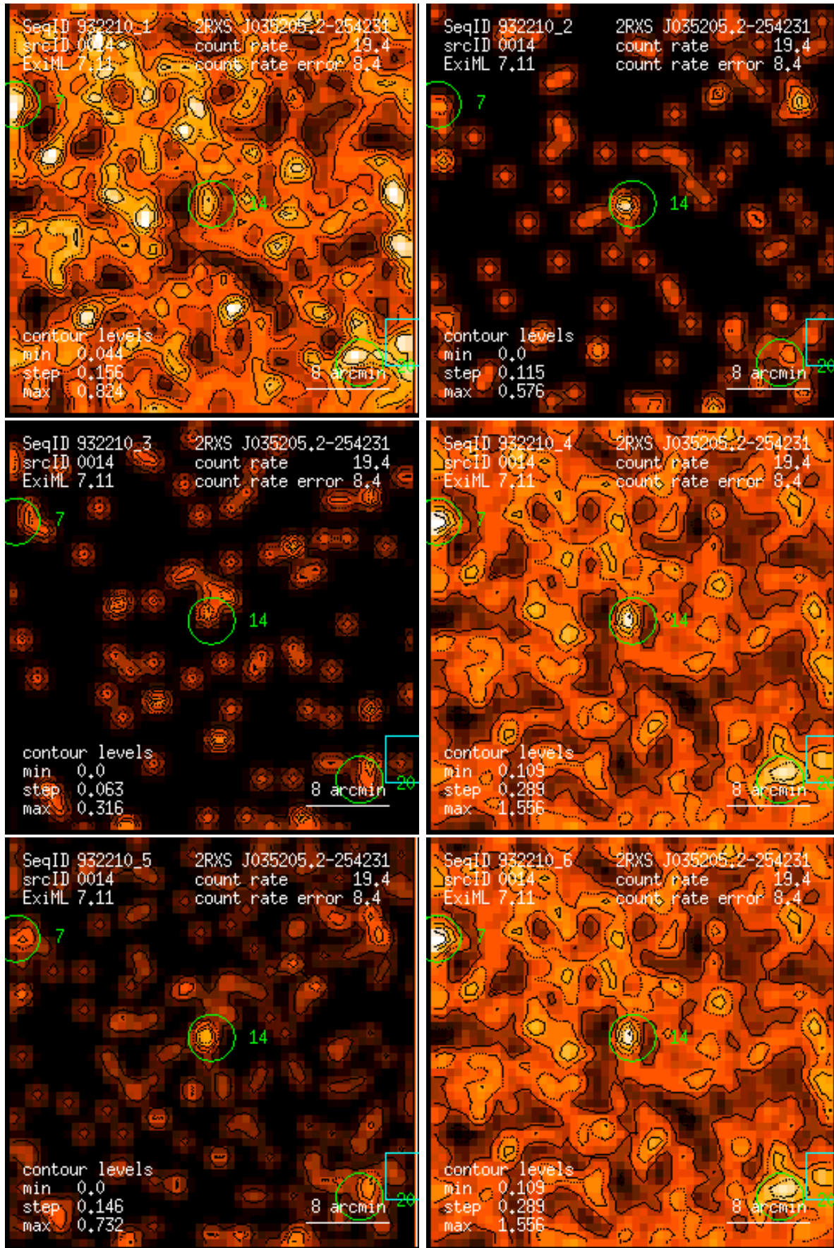
Figure 14: RASS 932210: detection 0014: band rate images, Gaussian filter: (1) PSPC channels 11 – 41, (2) 52 – 90, (3) 91 – 201, (4) 11 – 235, (5) 52 – 201, (6) 11 – 201. Broad band rates in counts/ks. Band rate contour levels in counts/ks/arcmin 2 .
