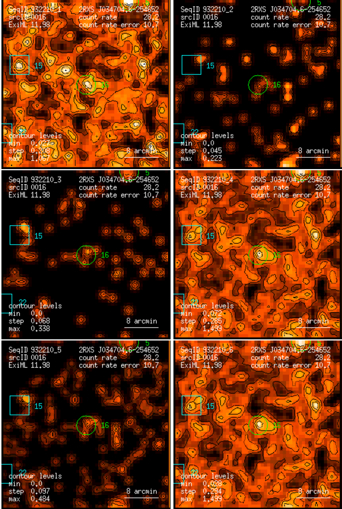
Figure 16: RASS 932210: detection 0016: band rate images, Gaussian filter: (1) PSPC channels 11 – 41, (2) 52 – 90, (3) 91 – 201, (4) 11 – 235, (5) 52 – 201, (6) 11 – 201. Broad band rates in counts/ks. Band rate contour levels in counts/ks/arcmin 2 .
