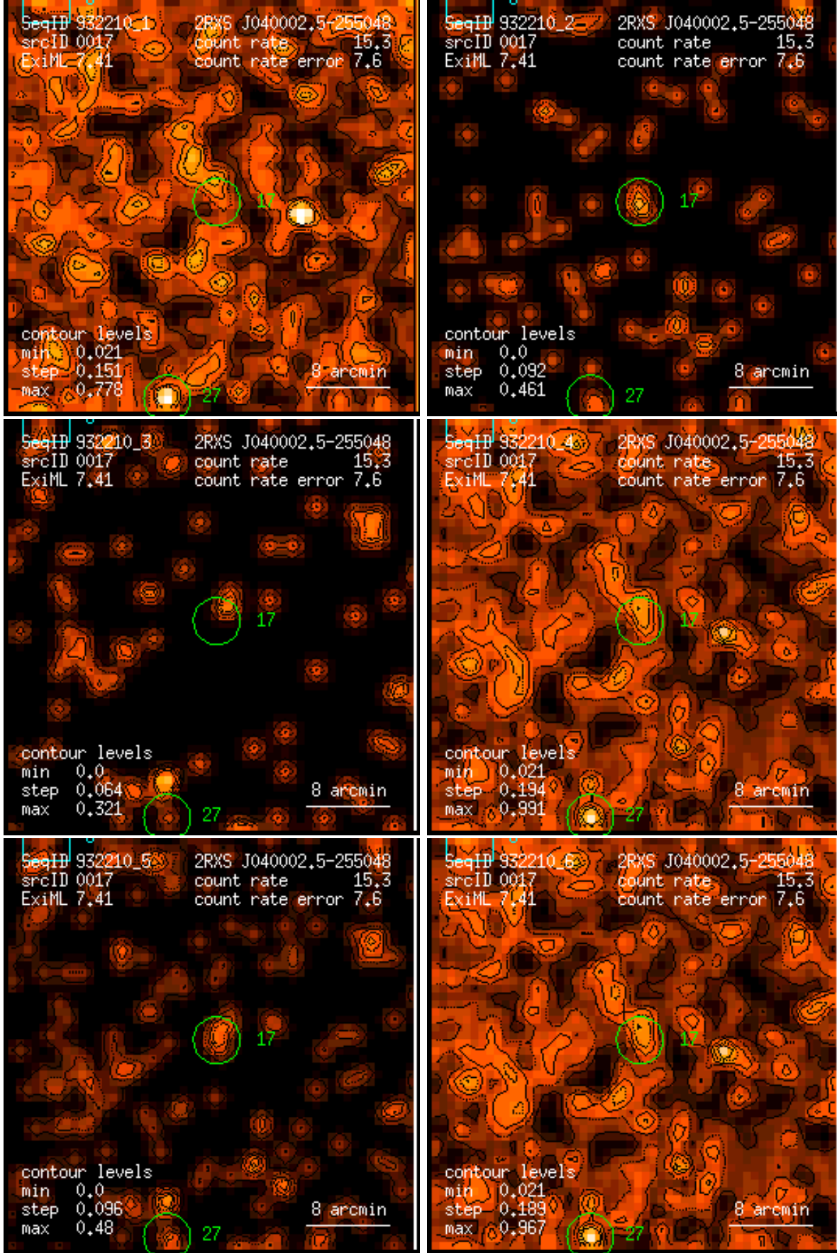
Figure 17: RASS 932210: detection 0017: band rate images, Gaussian filter: (1) PSPC channels 11 – 41, (2) 52 – 90, (3) 91 – 201, (4) 11 – 235, (5) 52 – 201, (6) 11 – 201. Broad band rates in counts/ks. Band rate contour levels in counts/ks/arcmin 2 .
