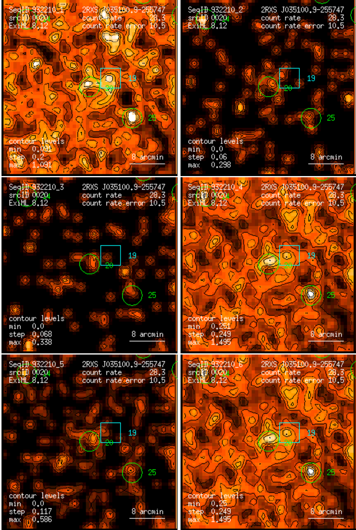
Figure 20: RASS 932210: detection 0020: band rate images, Gaussian filter: (1) PSPC channels 11 – 41, (2) 52 – 90, (3) 91 – 201, (4) 11 – 235, (5) 52 – 201, (6) 11 – 201. Broad band rates in counts/ks. Band rate contour levels in counts/ks/arcmin 2 .
