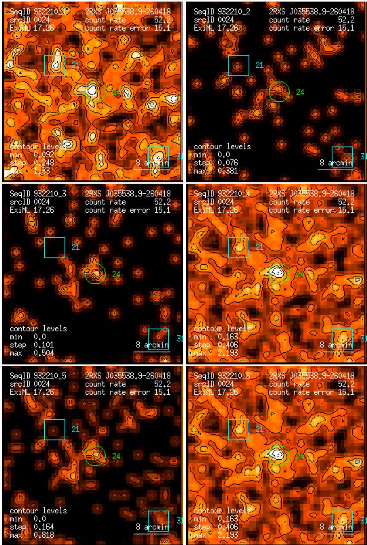
Figure 24: RASS 932210: detection 0024: band rate images, Gaussian filter: (1) PSPC channels 11 – 41, (2) 52 – 90, (3) 91 – 201, (4) 11 – 235, (5) 52 – 201, (6) 11 – 201. Broad band rates in counts/ks. Band rate contour levels in counts/ks/arcmin 2 .
