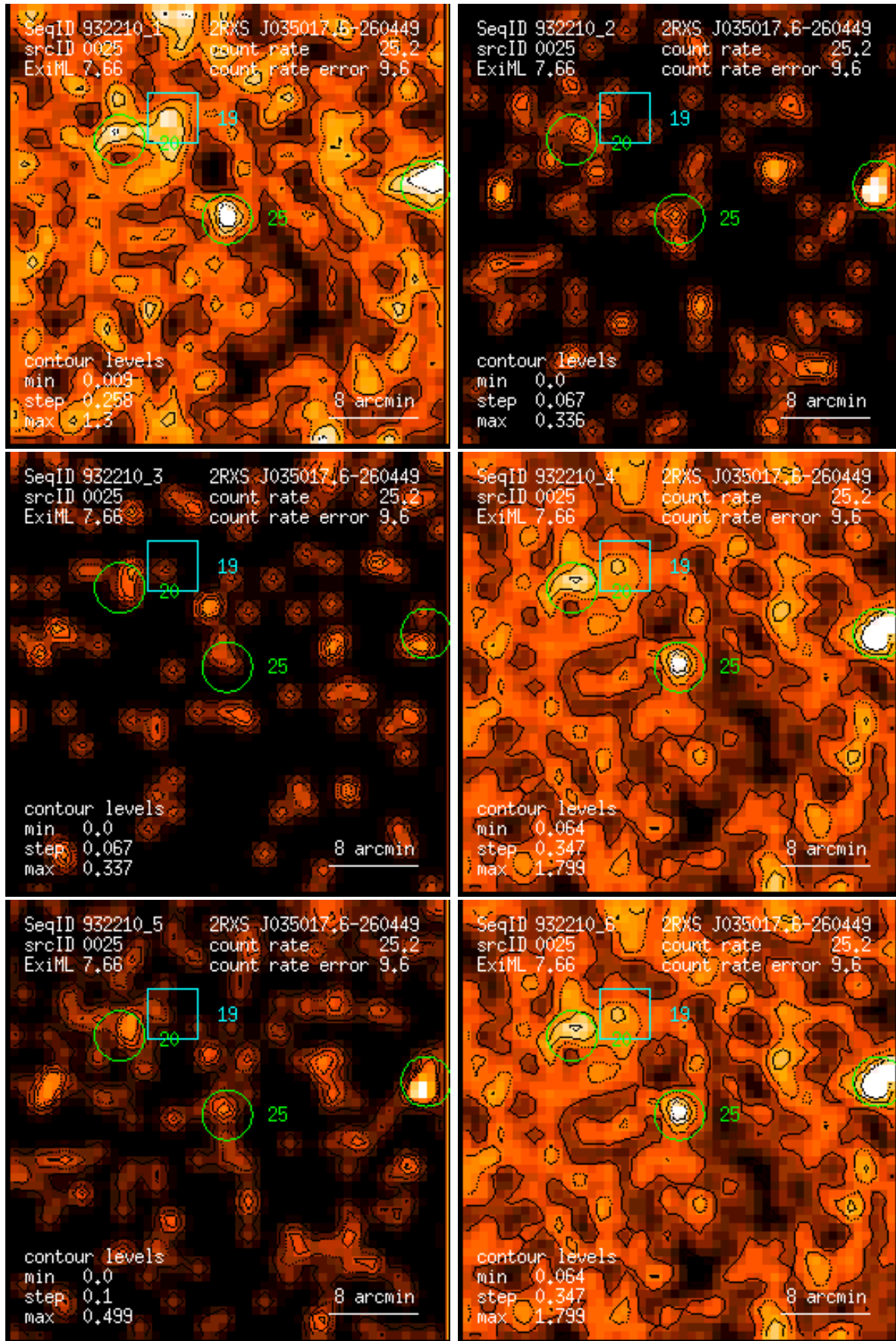
Figure 25: RASS 932210: detection 0025: band rate images, Gaussian filter: (1) PSPC channels 11 – 41, (2) 52 – 90, (3) 91 – 201, (4) 11 – 235, (5) 52 – 201, (6) 11 – 201. Broad band rates in counts/ks. Band rate contour levels in counts/ks/arcmin 2 .
