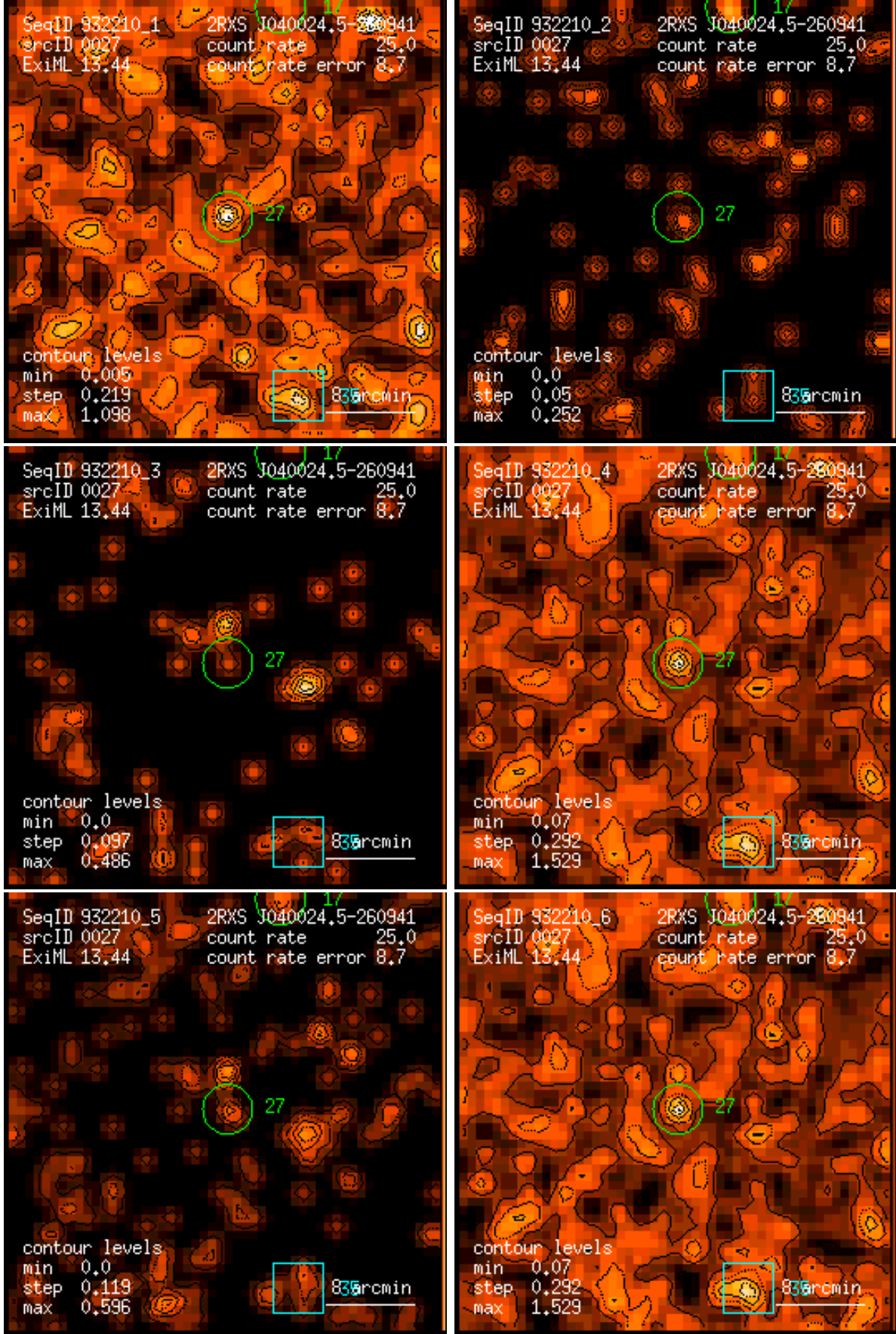
Figure 27: RASS 932210: detection 0027: band rate images, Gaussian filter: (1) PSPC channels 11 – 41, (2) 52 – 90, (3) 91 – 201, (4) 11 – 235, (5) 52 – 201, (6) 11 – 201. Broad band rates in counts/ks. Band rate contour levels in counts/ks/arcmin 2 .
