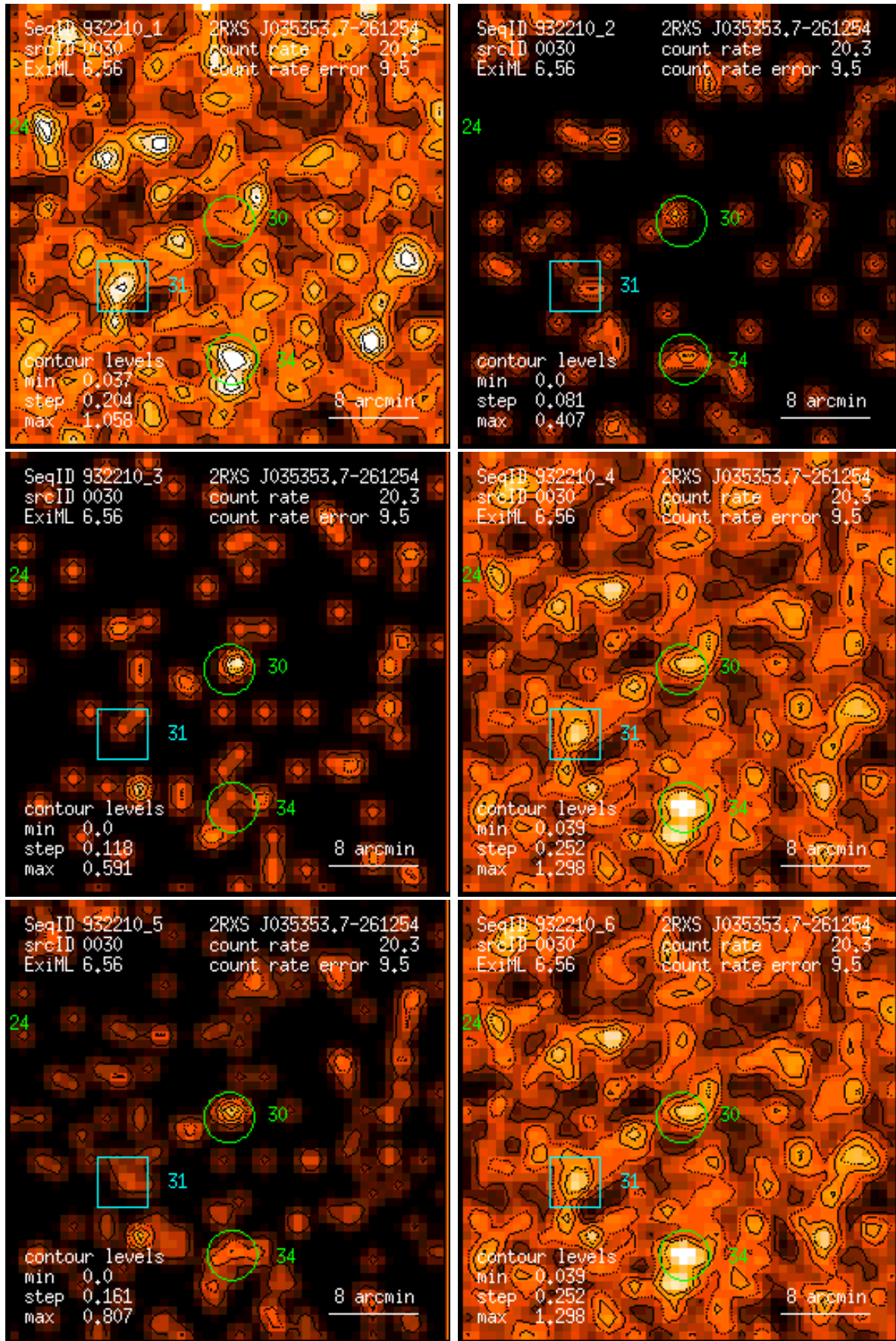
Figure 30: RASS 932210: detection 0030: band rate images, Gaussian filter: (1) PSPC channels 11 – 41, (2) 52 – 90, (3) 91 – 201, (4) 11 – 235, (5) 52 – 201, (6) 11 – 201. Broad band rates in counts/ks. Band rate contour levels in counts/ks/arcmin 2 .
