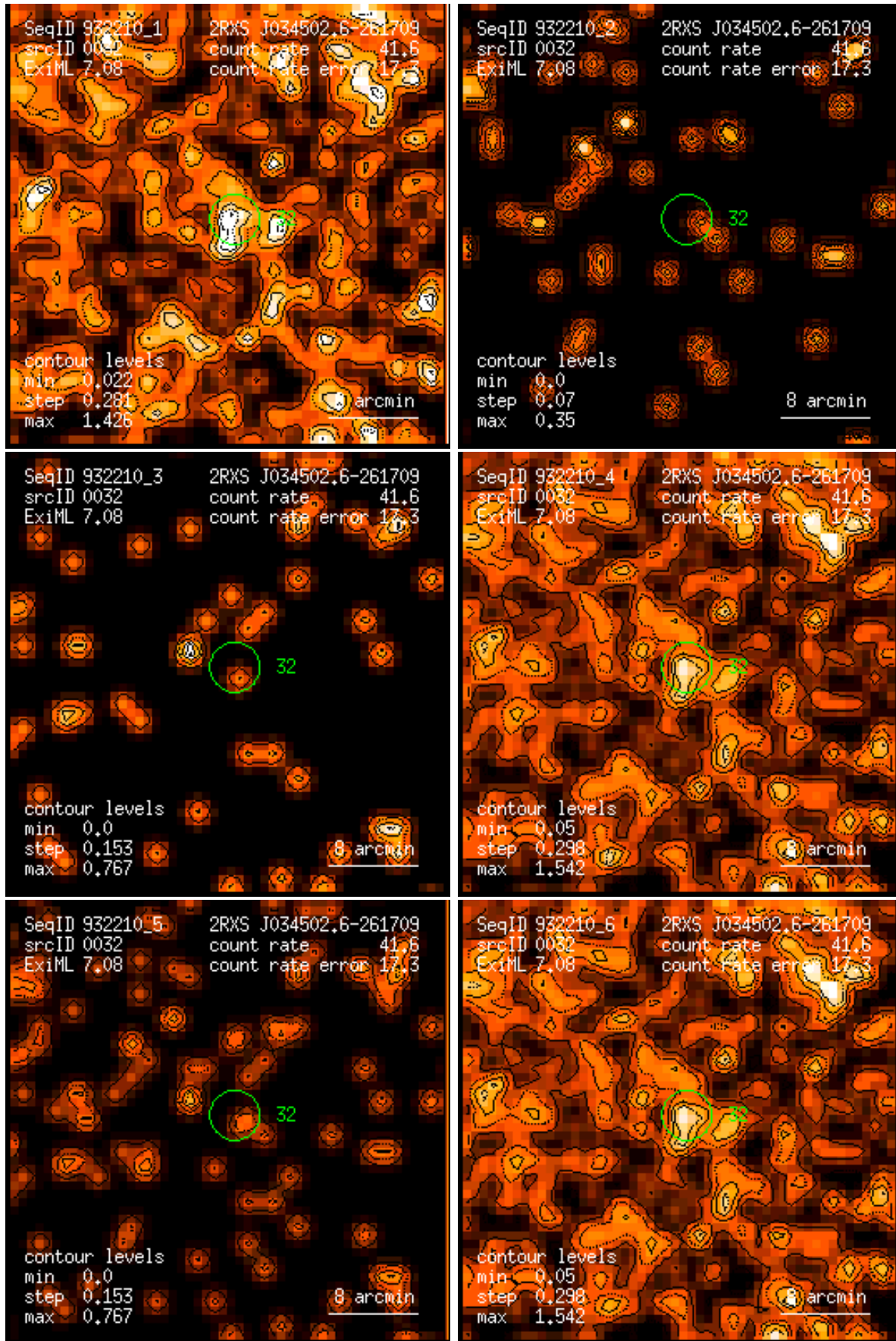
Figure 32: RASS 932210: detection 0032: band rate images, Gaussian filter: (1) PSPC channels 11 – 41, (2) 52 – 90, (3) 91 – 201, (4) 11 – 235, (5) 52 – 201, (6) 11 – 201. Broad band rates in counts/ks. Band rate contour levels in counts/ks/arcmin 2 .
