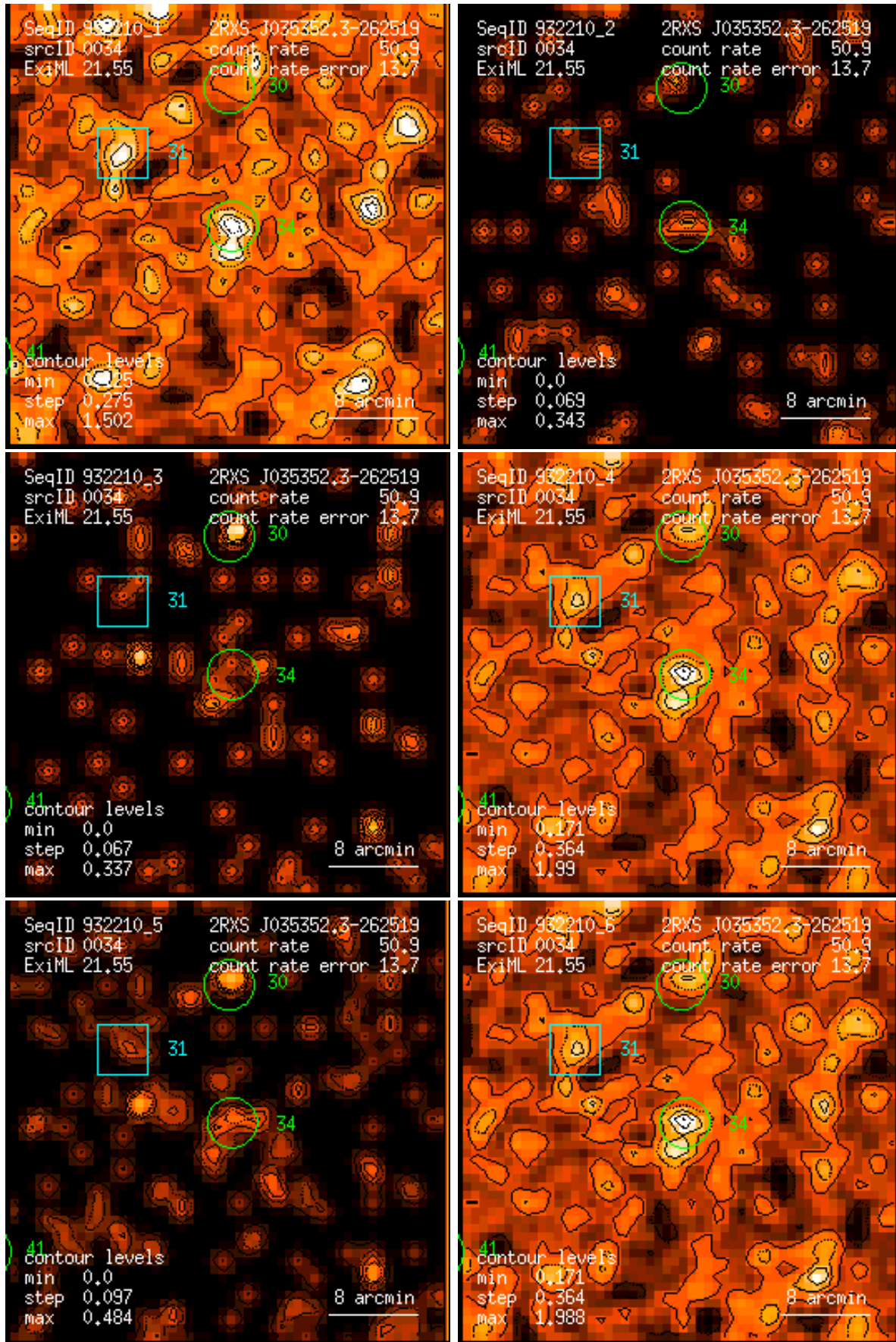
Figure 34: RASS 932210: detection 0034: band rate images, Gaussian filter: (1) PSPC channels 11 – 41, (2) 52 – 90, (3) 91 – 201, (4) 11 – 235, (5) 52 – 201, (6) 11 – 201. Broad band rates in counts/ks. Band rate contour levels in counts/ks/arcmin 2 .
