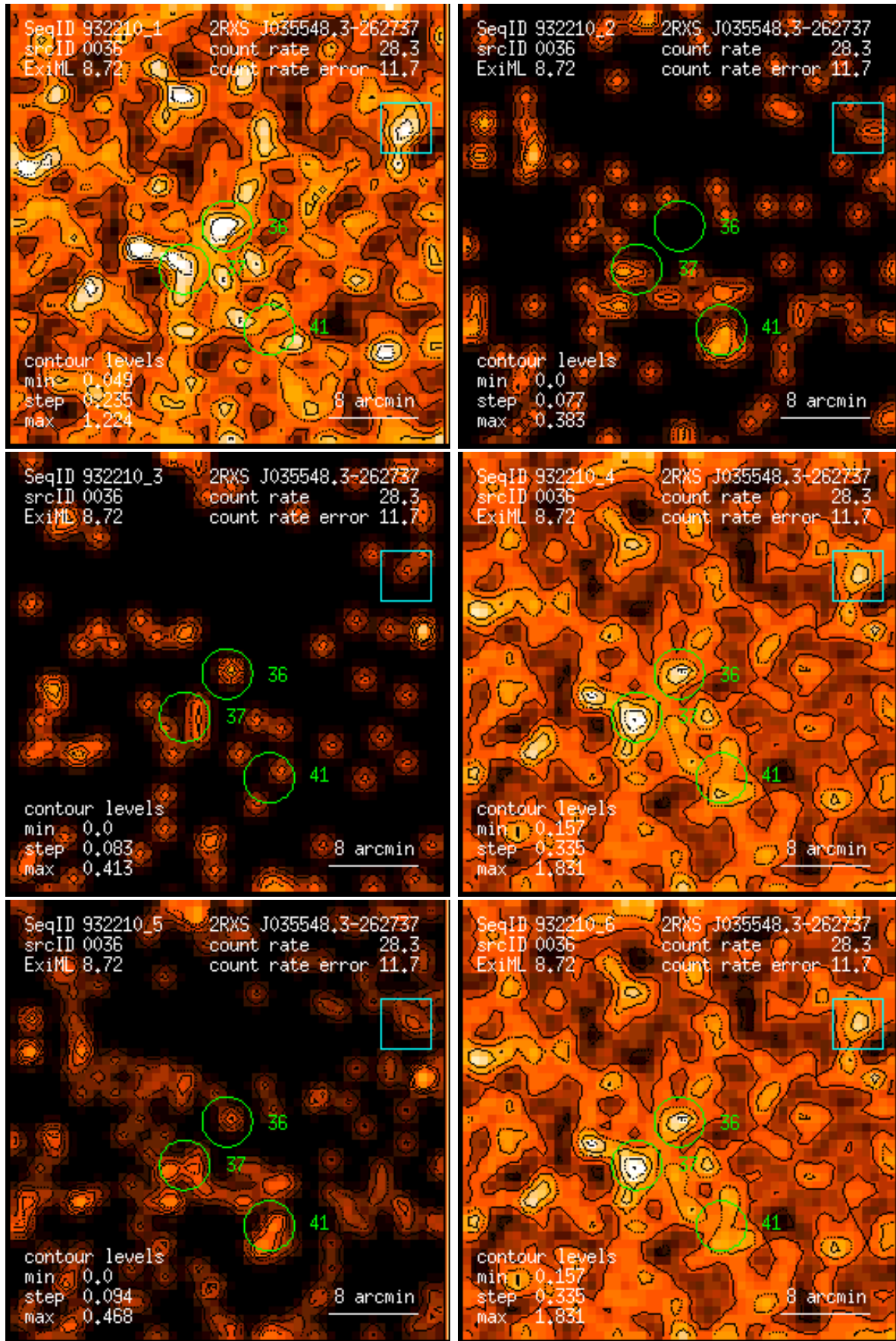
Figure 36: RASS 932210: detection 0036: band rate images, Gaussian filter: (1) PSPC channels 11 – 41, (2) 52 – 90, (3) 91 – 201, (4) 11 – 235, (5) 52 – 201, (6) 11 – 201. Broad band rates in counts/ks. Band rate contour levels in counts/ks/arcmin 2 .
