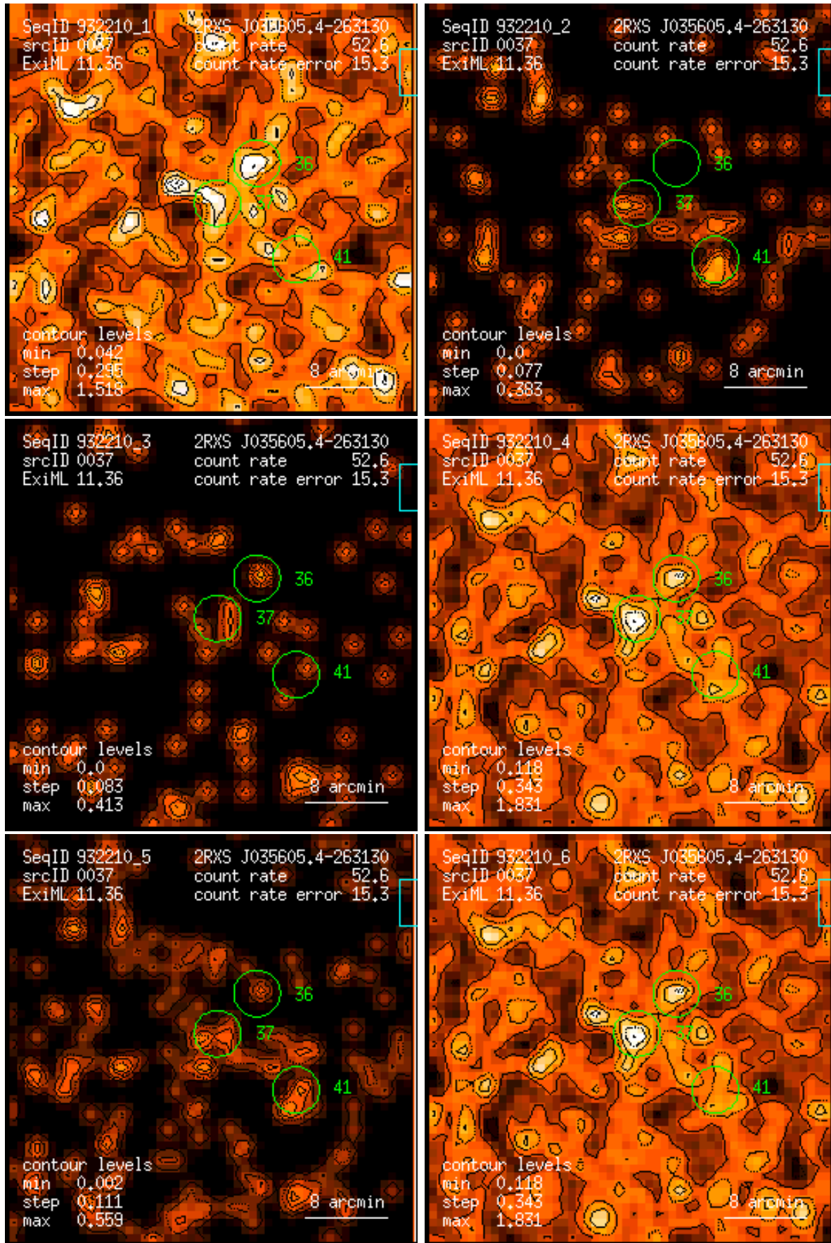
Figure 37: RASS 932210: detection 0037: band rate images, Gaussian filter: (1) PSPC channels 11 – 41, (2) 52 – 90, (3) 91 – 201, (4) 11 – 235, (5) 52 – 201, (6) 11 – 201. Broad band rates in counts/ks. Band rate contour levels in counts/ks/arcmin 2 .
