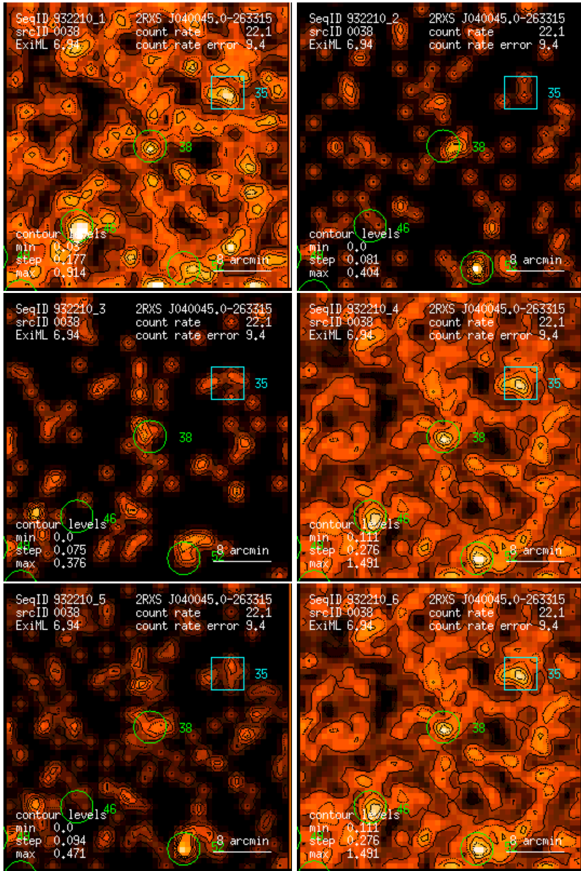
Figure 38: RASS 932210: detection 0038: band rate images, Gaussian filter: (1) PSPC channels 11 – 41, (2) 52 – 90, (3) 91 – 201, (4) 11 – 235, (5) 52 – 201, (6) 11 – 201. Broad band rates in counts/ks. Band rate contour levels in counts/ks/arcmin 2 .
