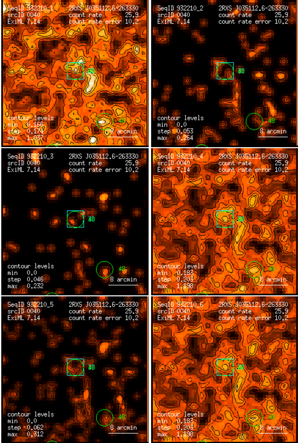
Figure 40: RASS 932210: detection 0040: band rate images, Gaussian filter: (1) PSPC channels 11 – 41, (2) 52 – 90, (3) 91 – 201, (4) 11 – 235, (5) 52 – 201, (6) 11 – 201. Broad band rates in counts/ks. Band rate contour levels in counts/ks/arcmin 2 .
