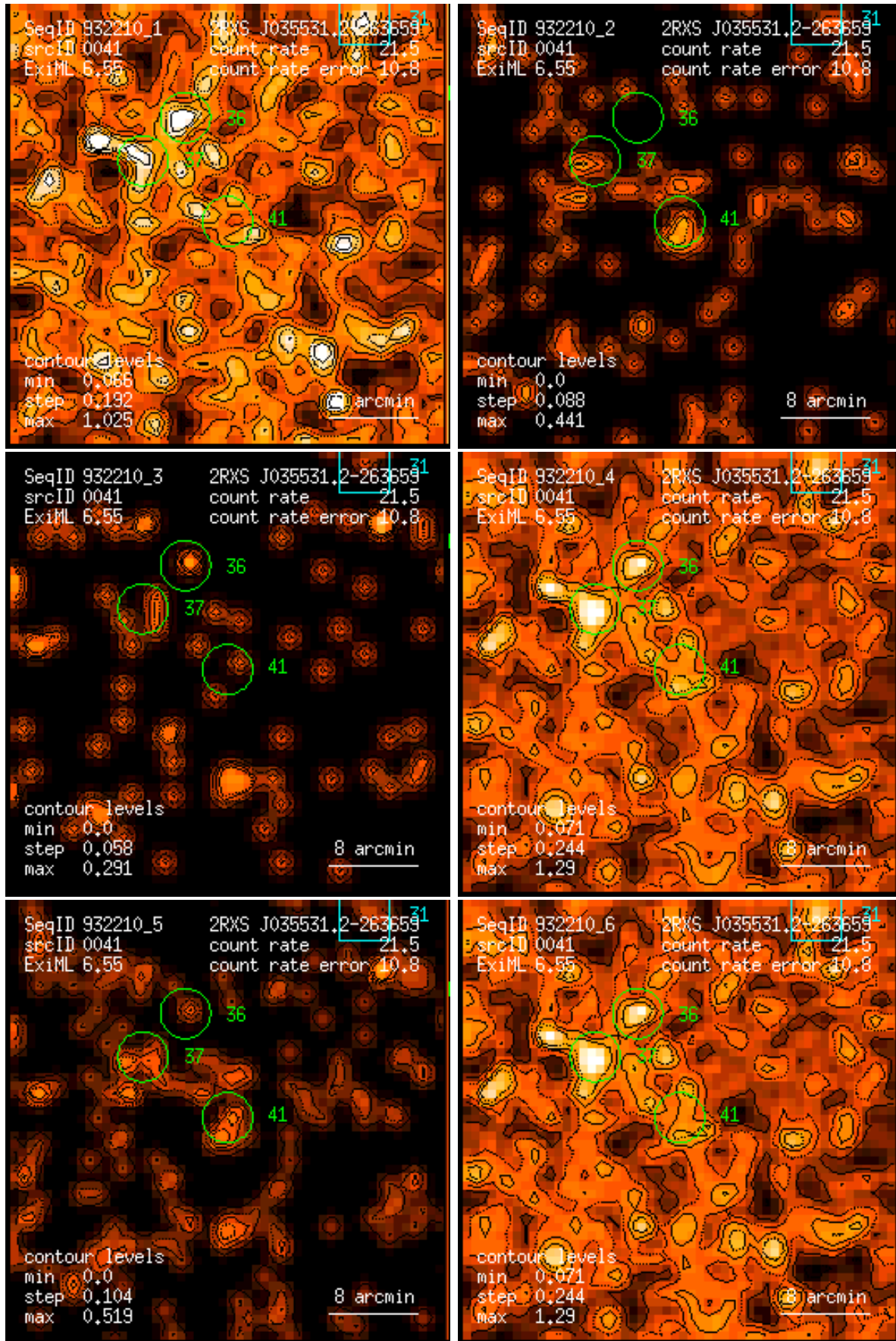
Figure 41: RASS 932210: detection 0041: band rate images, Gaussian filter: (1) PSPC channels 11 – 41, (2) 52 – 90, (3) 91 – 201, (4) 11 – 235, (5) 52 – 201, (6) 11 – 201. Broad band rates in counts/ks. Band rate contour levels in counts/ks/arcmin 2 .
