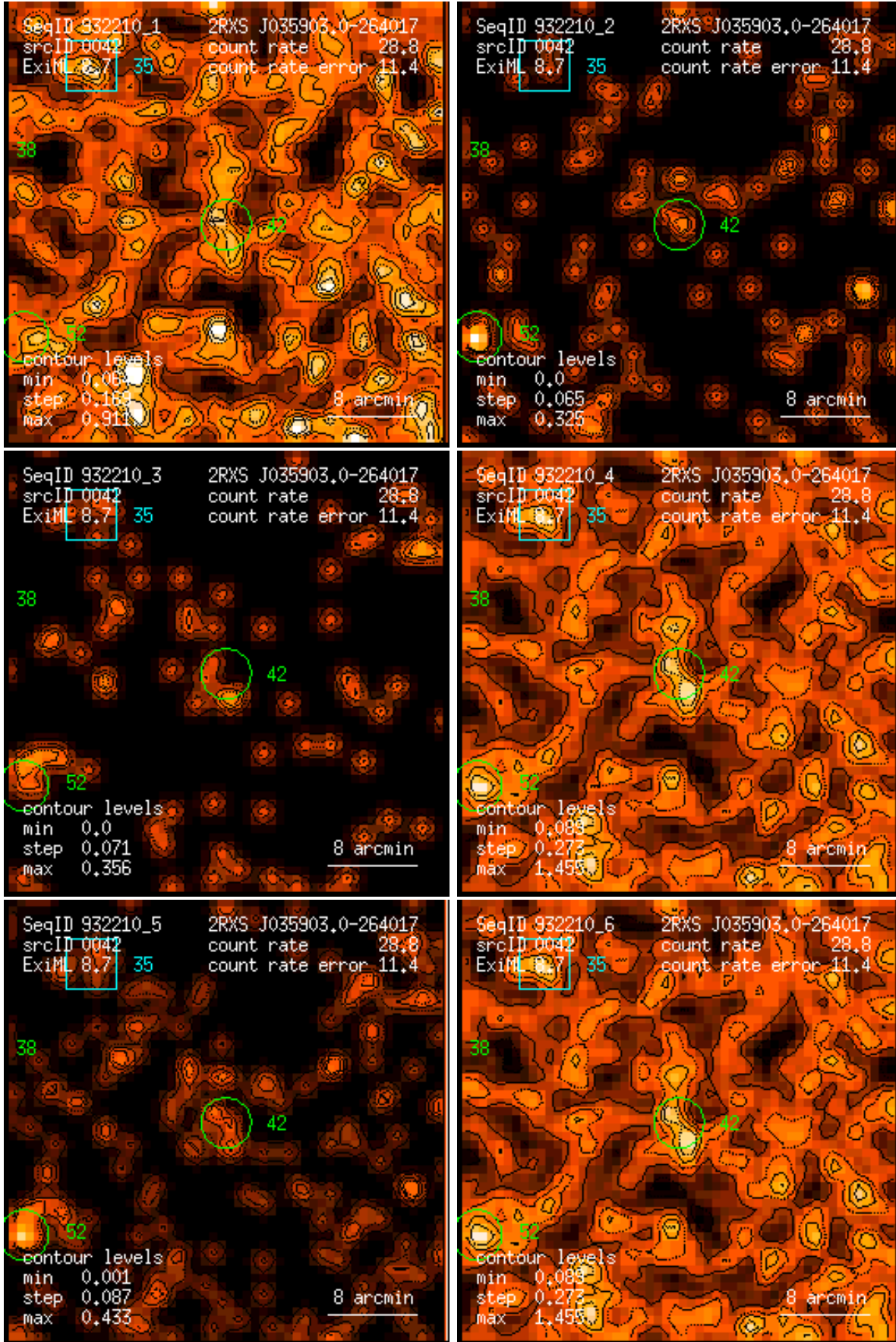
Figure 42: RASS 932210: detection 0042: band rate images, Gaussian filter: (1) PSPC channels 11 – 41, (2) 52 – 90, (3) 91 – 201, (4) 11 – 235, (5) 52 – 201, (6) 11 – 201. Broad band rates in counts/ks. Band rate contour levels in counts/ks/arcmin 2 .
