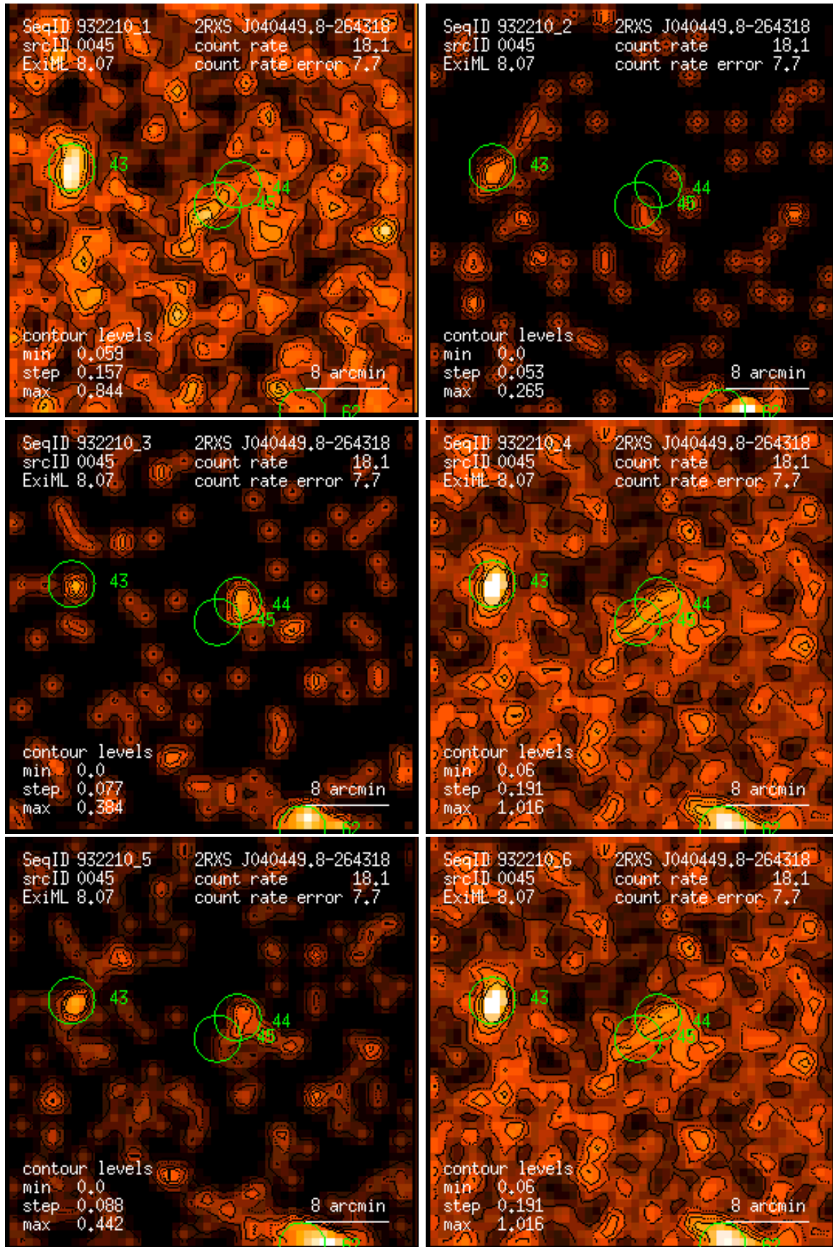
Figure 45: RASS 932210: detection 0045: band rate images, Gaussian filter: (1) PSPC channels 11 – 41, (2) 52 – 90, (3) 91 – 201, (4) 11 – 235, (5) 52 – 201, (6) 11 – 201. Broad band rates in counts/ks. Band rate contour levels in counts/ks/arcmin 2 .
