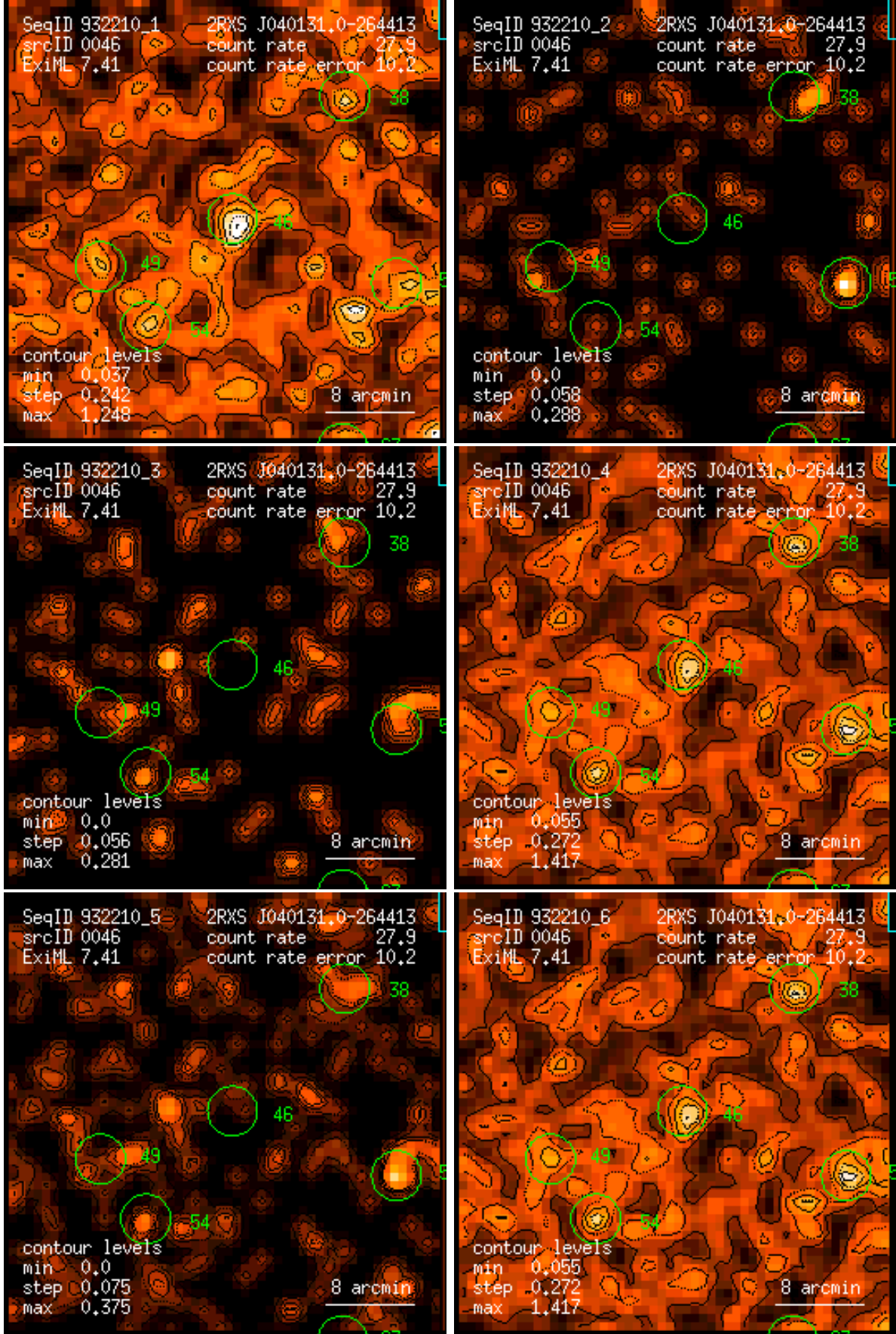
Figure 46: RASS 932210: detection 0046: band rate images, Gaussian filter: (1) PSPC channels 11 – 41, (2) 52 – 90, (3) 91 – 201, (4) 11 – 235, (5) 52 – 201, (6) 11 – 201. Broad band rates in counts/ks. Band rate contour levels in counts/ks/arcmin 2 .
