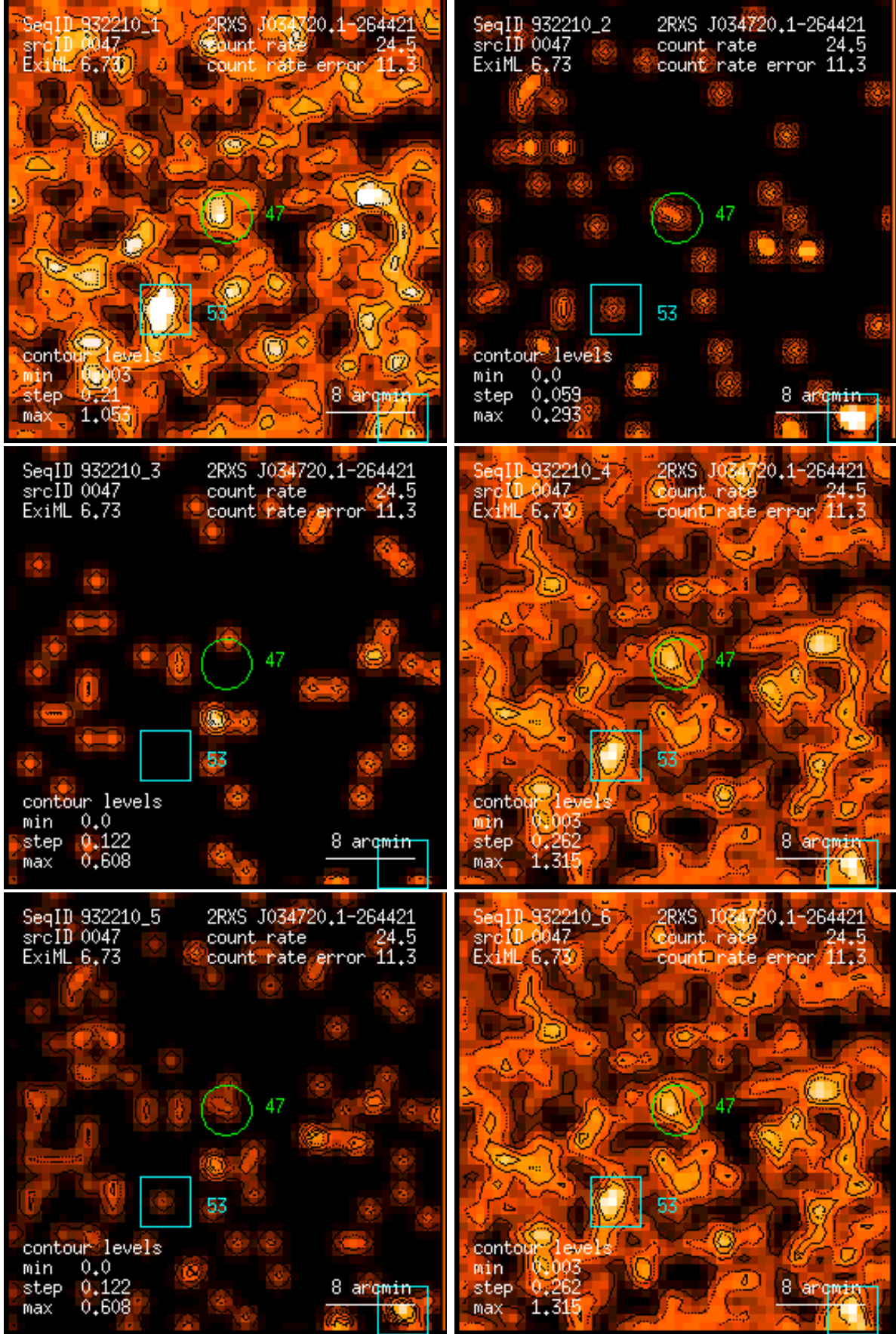
Figure 47: RASS 932210: detection 0047: band rate images, Gaussian filter: (1) PSPC channels 11 – 41, (2) 52 – 90, (3) 91 – 201, (4) 11 – 235, (5) 52 – 201, (6) 11 – 201. Broad band rates in counts/ks. Band rate contour levels in counts/ks/arcmin 2 .
