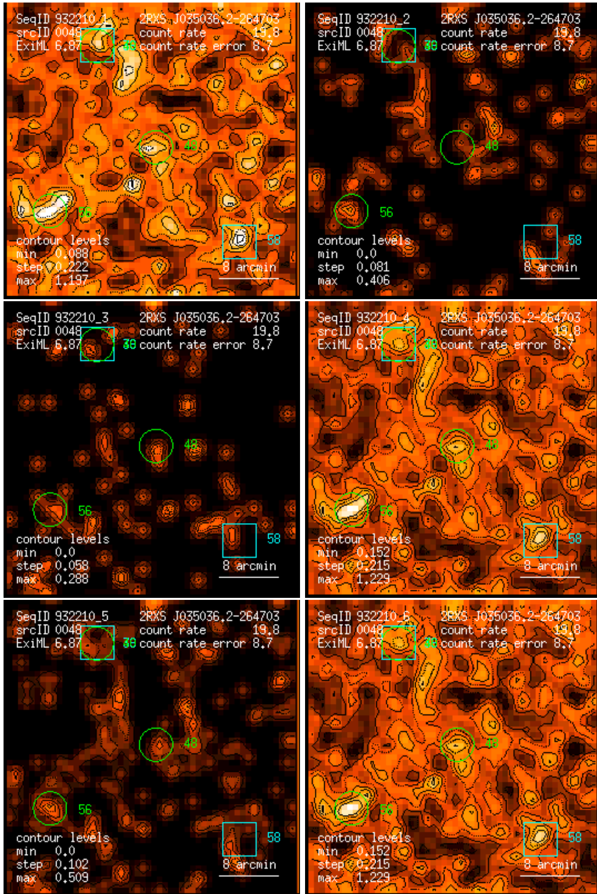
Figure 48: RASS 932210: detection 0048: band rate images, Gaussian filter: (1) PSPC channels 11 – 41, (2) 52 – 90, (3) 91 – 201, (4) 11 – 235, (5) 52 – 201, (6) 11 – 201. Broad band rates in counts/ks. Band rate contour levels in counts/ks/arcmin 2 .
