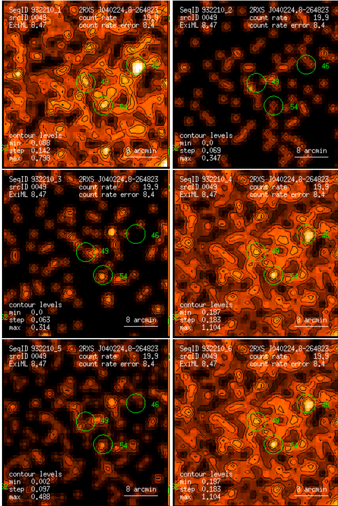
Figure 49: RASS 932210: detection 0049: band rate images, Gaussian filter: (1) PSPC channels 11 – 41, (2) 52 – 90, (3) 91 – 201, (4) 11 – 235, (5) 52 – 201, (6) 11 – 201. Broad band rates in counts/ks. Band rate contour levels in counts/ks/arcmin 2 .
