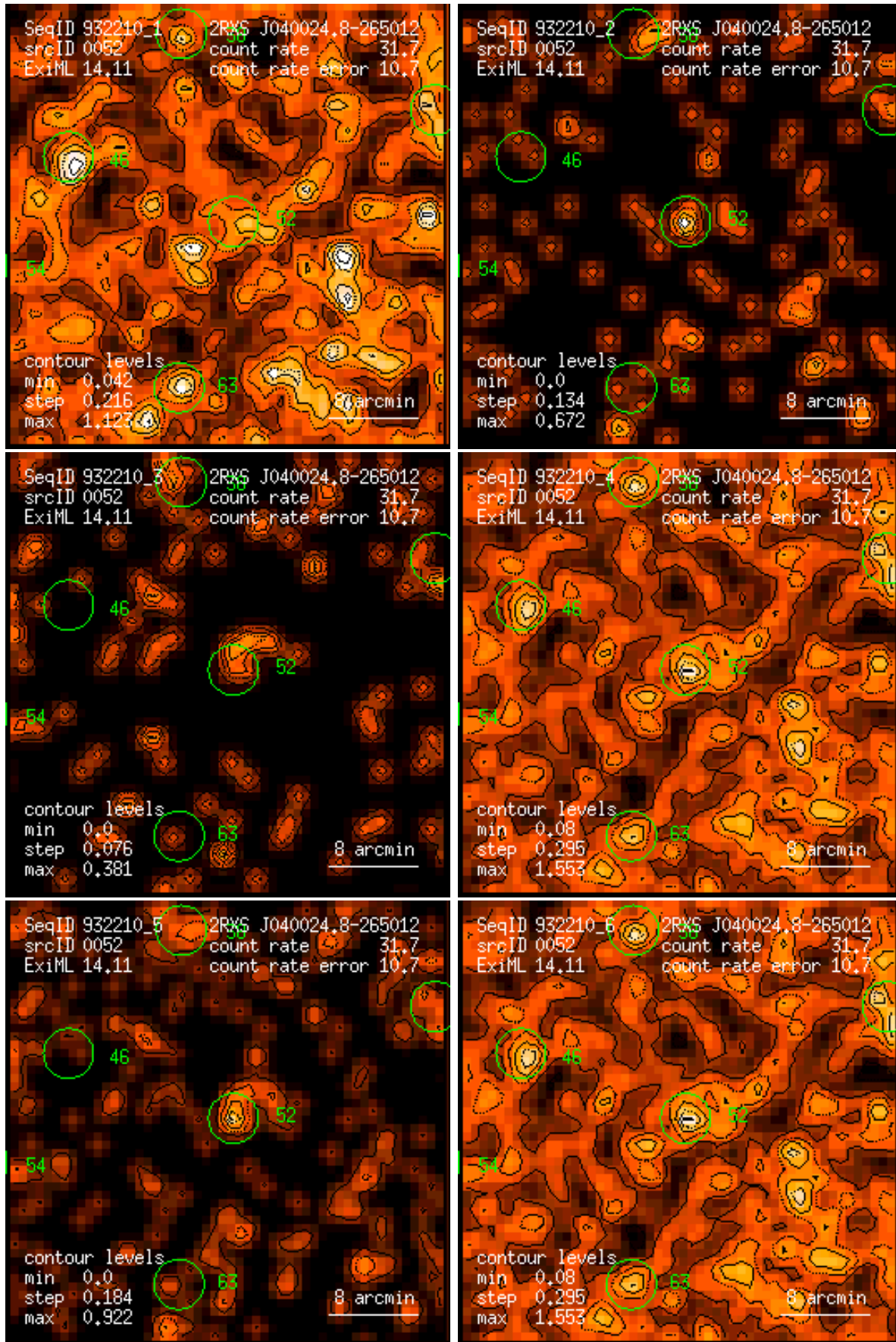
Figure 52: RASS 932210: detection 0052: band rate images, Gaussian filter: (1) PSPC channels 11 – 41, (2) 52 – 90, (3) 91 – 201, (4) 11 – 235, (5) 52 – 201, (6) 11 – 201. Broad band rates in counts/ks. Band rate contour levels in counts/ks/arcmin 2 .
