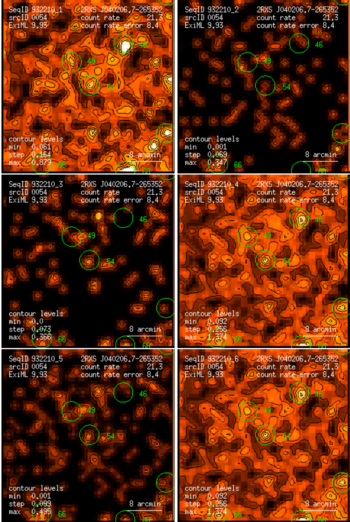
Figure 54: RASS 932210: detection 0054: band rate images, Gaussian filter: (1) PSPC channels 11 – 41, (2) 52 – 90, (3) 91 – 201, (4) 11 – 235, (5) 52 – 201, (6) 11 – 201. Broad band rates in counts/ks. Band rate contour levels in counts/ks/arcmin 2 .
