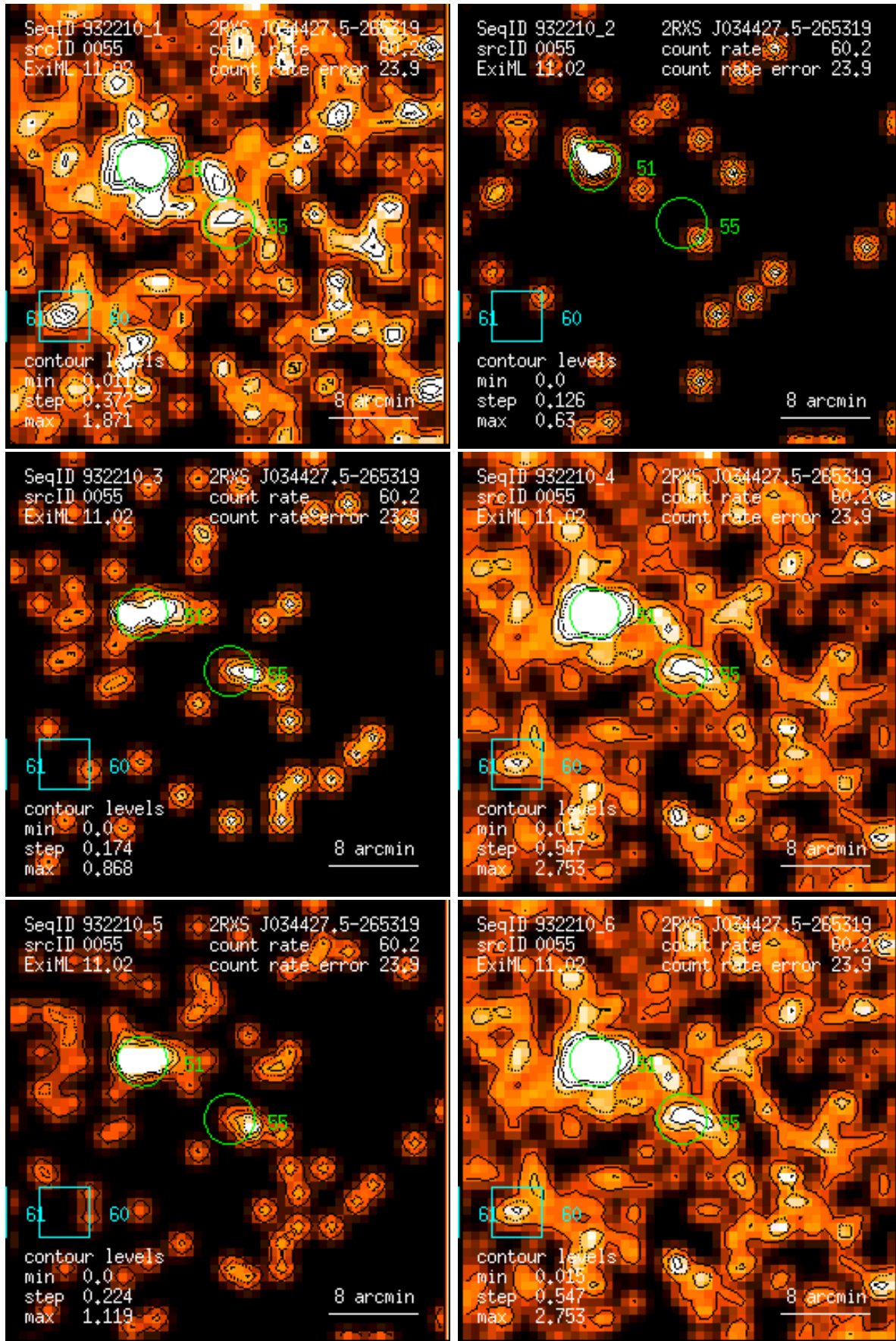
Figure 55: RASS 932210: detection 0055: band rate images, Gaussian filter: (1) PSPC channels 11 – 41, (2) 52 – 90, (3) 91 – 201, (4) 11 – 235, (5) 52 – 201, (6) 11 – 201. Broad band rates in counts/ks. Band rate contour levels in counts/ks/arcmin 2 .
