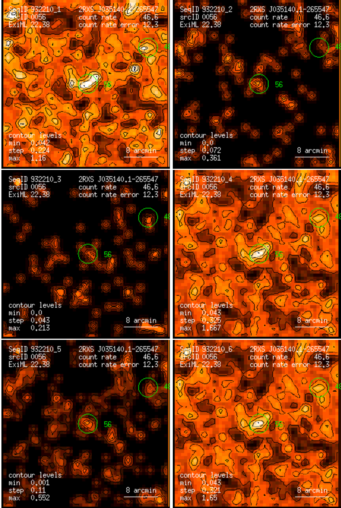
Figure 56: RASS 932210: detection 0056: band rate images, Gaussian filter: (1) PSPC channels 11 – 41, (2) 52 – 90, (3) 91 – 201, (4) 11 – 235, (5) 52 – 201, (6) 11 – 201. Broad band rates in counts/ks. Band rate contour levels in counts/ks/arcmin 2 .
