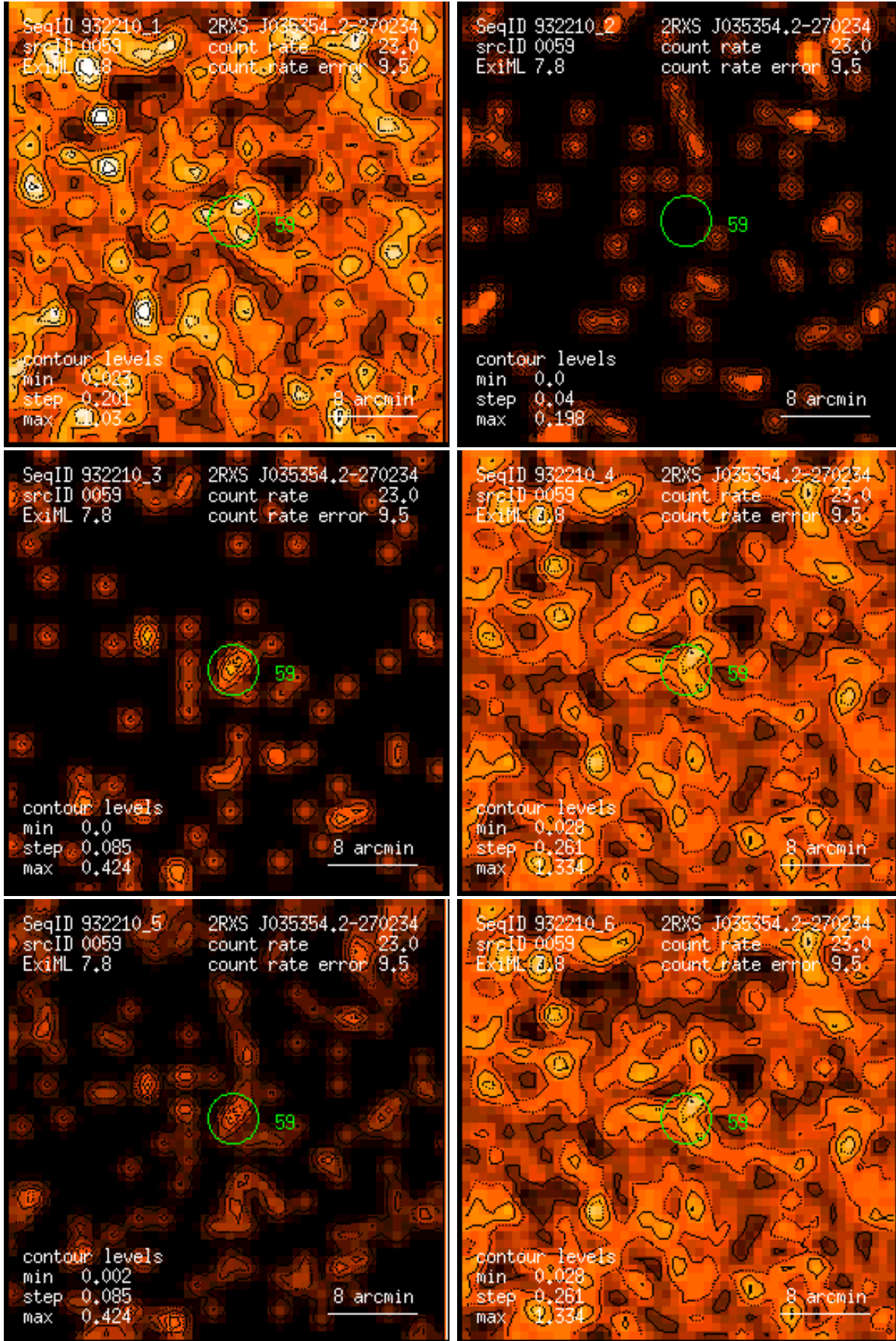
Figure 59: RASS 932210: detection 0059: band rate images, Gaussian filter: (1) PSPC channels 11 – 41, (2) 52 – 90, (3) 91 – 201, (4) 11 – 235, (5) 52 – 201, (6) 11 – 201. Broad band rates in counts/ks. Band rate contour levels in counts/ks/arcmin 2 .
