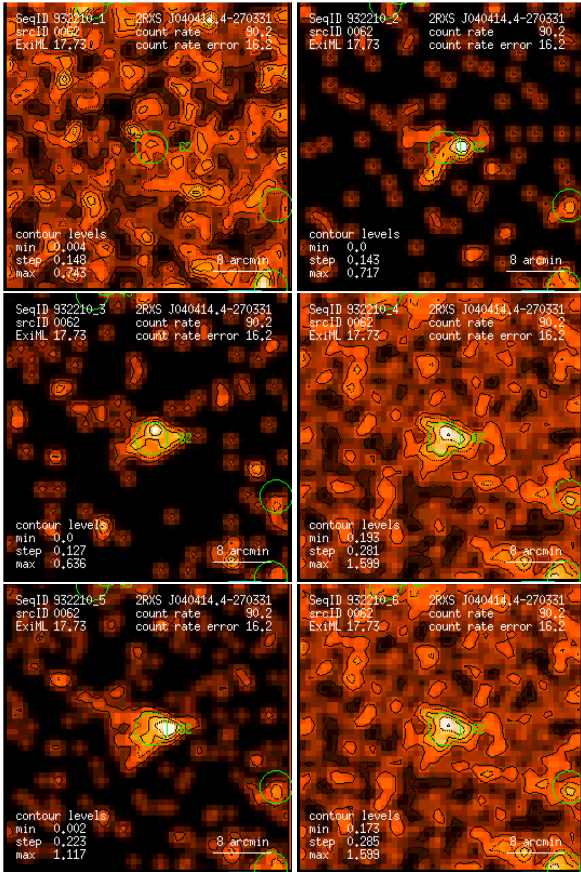
Figure 62: RASS 932210: detection 0062: band rate images, Gaussian filter: (1) PSPC channels 11 – 41, (2) 52 – 90, (3) 91 – 201, (4) 11 – 235, (5) 52 – 201, (6) 11 – 201. Broad band rates in counts/ks. Band rate contour levels in counts/ks/arcmin 2 .
