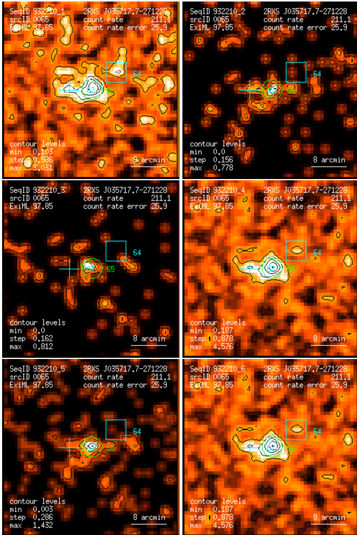
Figure 65: RASS 932210: detection 0065: band rate images, Gaussian filter: (1) PSPC channels 11 – 41, (2) 52 – 90, (3) 91 – 201, (4) 11 – 235, (5) 52 – 201, (6) 11 – 201. Broad band rates in counts/ks. Band rate contour levels in counts/ks/arcmin 2 .
