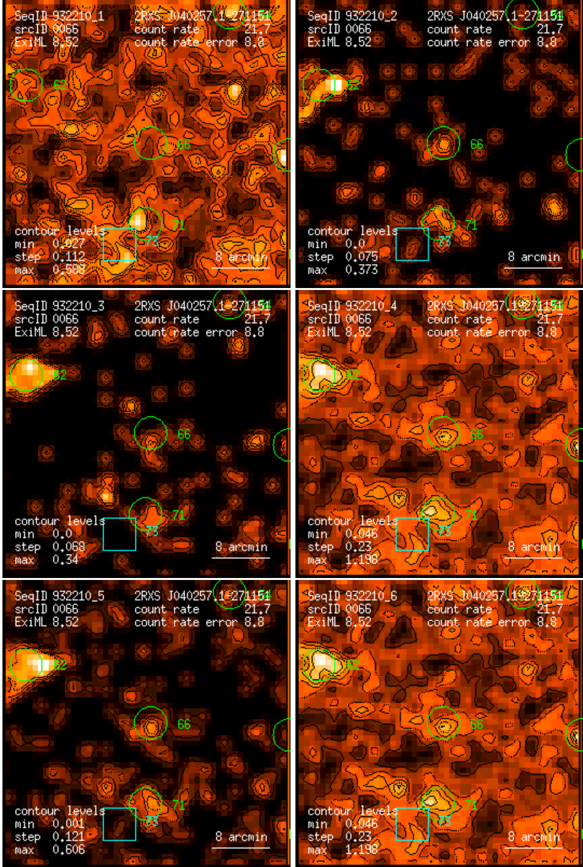
Figure 66: RASS 932210: detection 0066: band rate images, Gaussian filter: (1) PSPC channels 11 – 41, (2) 52 – 90, (3) 91 – 201, (4) 11 – 235, (5) 52 – 201, (6) 11 – 201. Broad band rates in counts/ks. Band rate contour levels in counts/ks/arcmin 2 .
