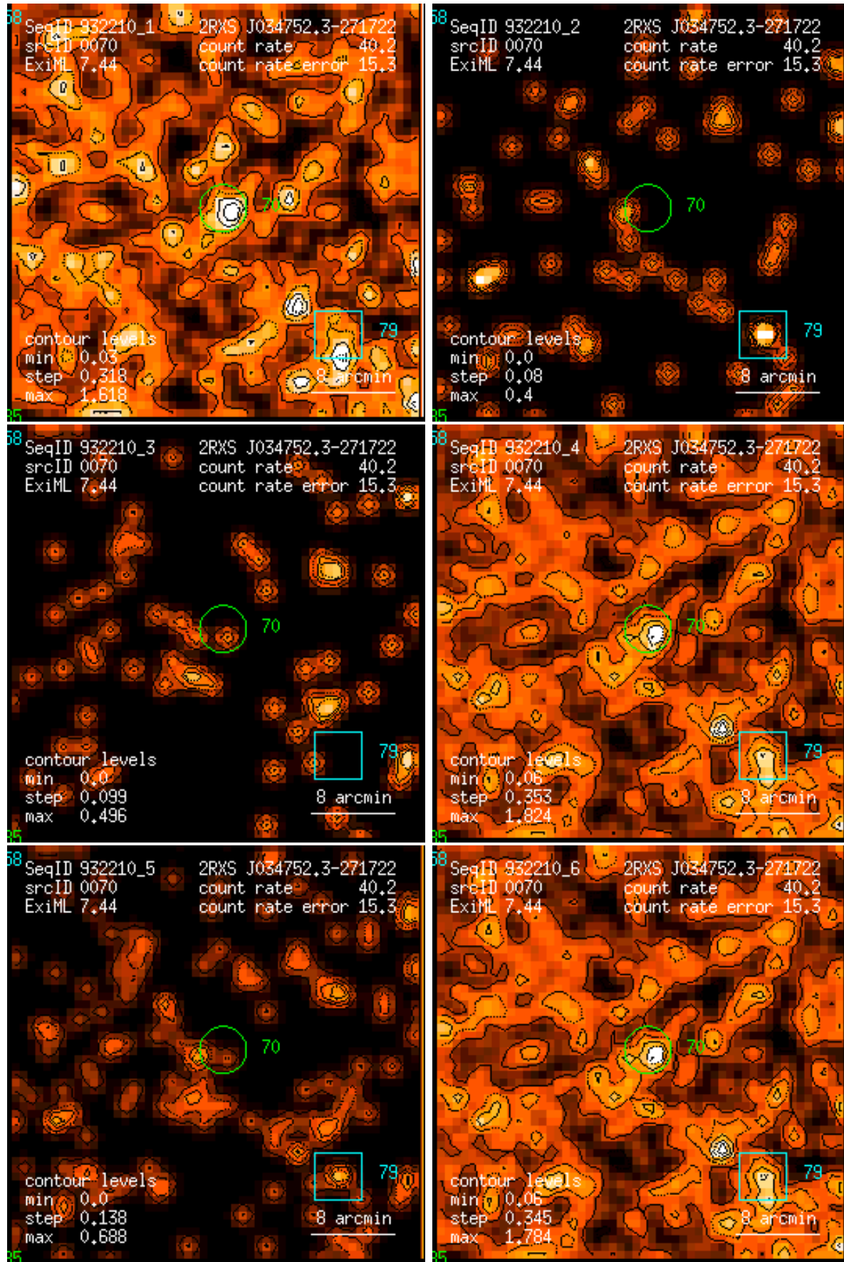
Figure 70: RASS 932210: detection 0070: band rate images, Gaussian filter: (1) PSPC channels 11 – 41, (2) 52 – 90, (3) 91 – 201, (4) 11 – 235, (5) 52 – 201, (6) 11 – 201. Broad band rates in counts/ks. Band rate contour levels in counts/ks/arcmin 2 .
