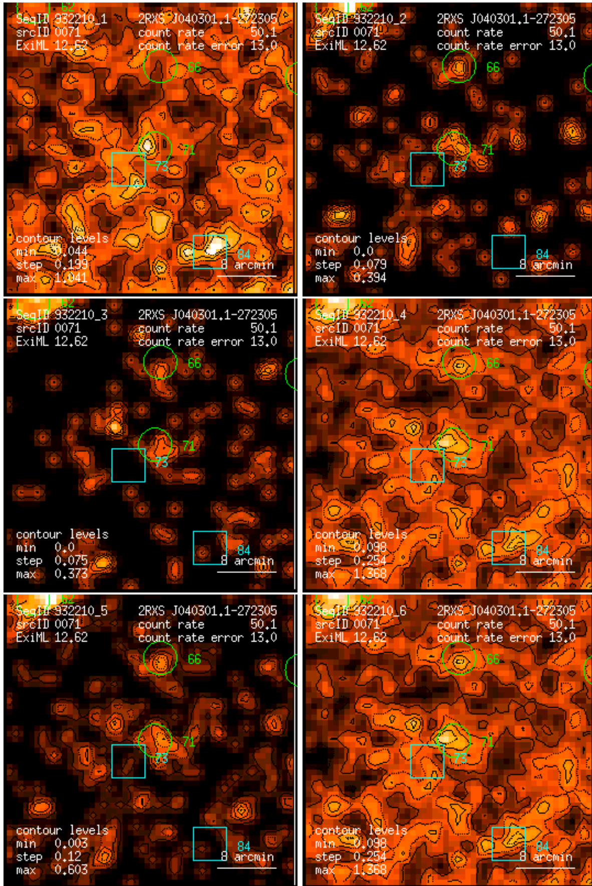
Figure 71: RASS 932210: detection 0071: band rate images, Gaussian filter: (1) PSPC channels 11 – 41, (2) 52 – 90, (3) 91 – 201, (4) 11 – 235, (5) 52 – 201, (6) 11 – 201. Broad band rates in counts/ks. Band rate contour levels in counts/ks/arcmin 2 .
