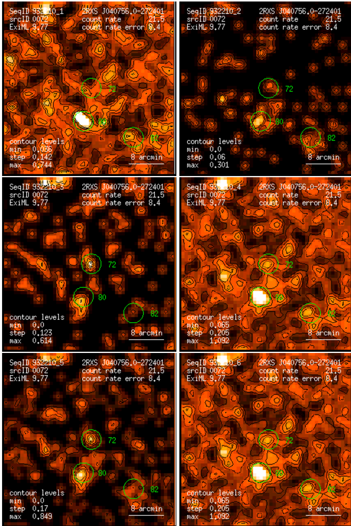
Figure 72: RASS 932210: detection 0072: band rate images, Gaussian filter: (1) PSPC channels 11 – 41, (2) 52 – 90, (3) 91 – 201, (4) 11 – 235, (5) 52 – 201, (6) 11 – 201. Broad band rates in counts/ks. Band rate contour levels in counts/ks/arcmin 2 .
