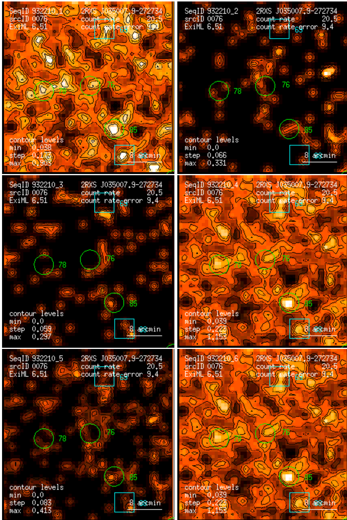
Figure 76: RASS 932210: detection 0076: band rate images, Gaussian filter: (1) PSPC channels 11 – 41, (2) 52 – 90, (3) 91 – 201, (4) 11 – 235, (5) 52 – 201, (6) 11 – 201. Broad band rates in counts/ks. Band rate contour levels in counts/ks/arcmin 2 .
