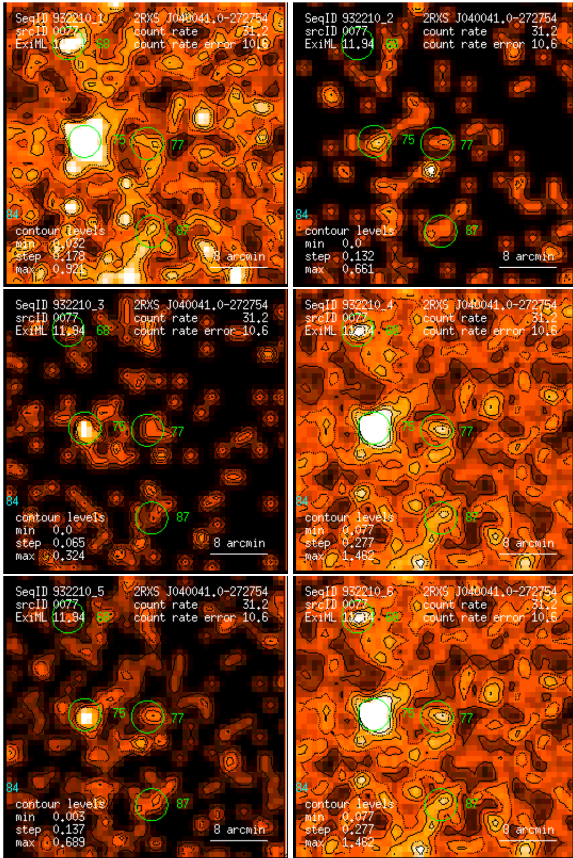
Figure 77: RASS 932210: detection 0077: band rate images, Gaussian filter: (1) PSPC channels 11 – 41, (2) 52 – 90, (3) 91 – 201, (4) 11 – 235, (5) 52 – 201, (6) 11 – 201. Broad band rates in counts/ks. Band rate contour levels in counts/ks/arcmin 2 .
