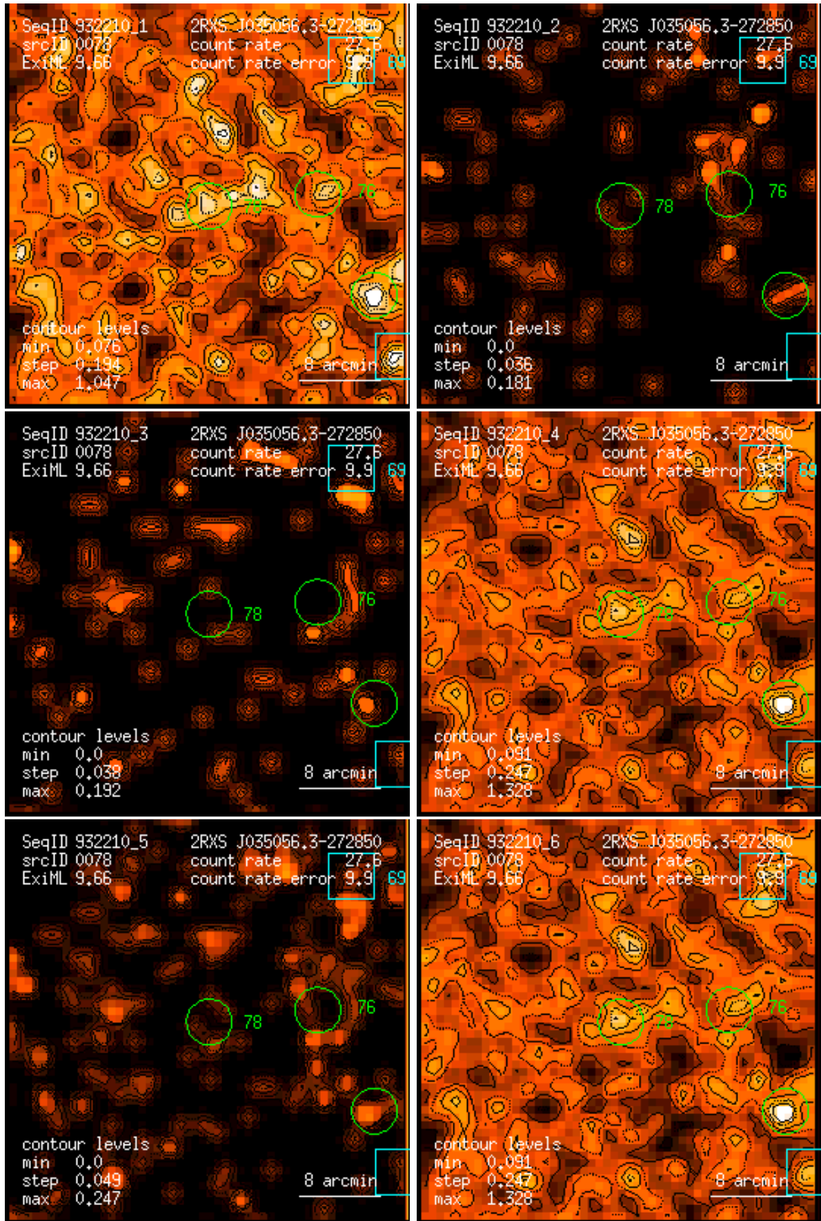
Figure 78: RASS 932210: detection 0078: band rate images, Gaussian filter: (1) PSPC channels 11 – 41, (2) 52 – 90, (3) 91 – 201, (4) 11 – 235, (5) 52 – 201, (6) 11 – 201. Broad band rates in counts/ks. Band rate contour levels in counts/ks/arcmin 2 .
