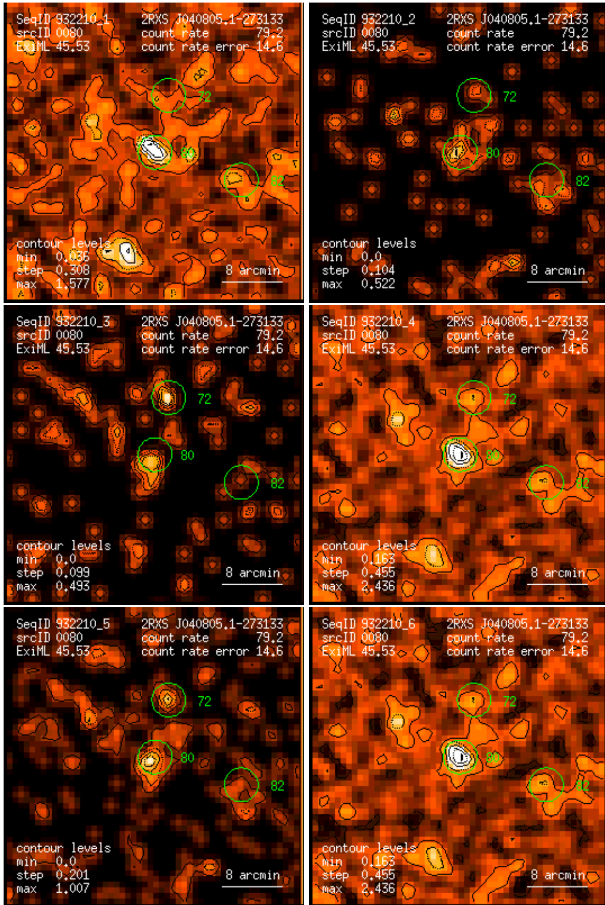
Figure 80: RASS 932210: detection 0080: band rate images, Gaussian filter: (1) PSPC channels 11 – 41, (2) 52 – 90, (3) 91 – 201, (4) 11 – 235, (5) 52 – 201, (6) 11 – 201. Broad band rates in counts/ks. Band rate contour levels in counts/ks/arcmin 2 .
