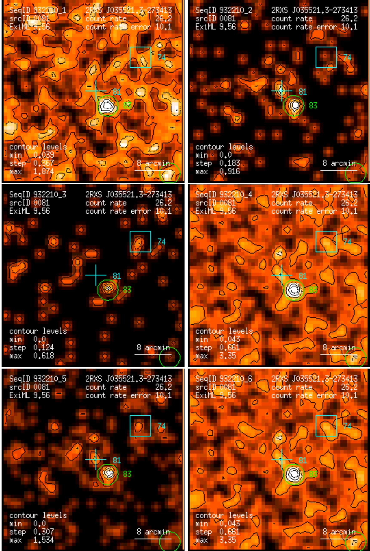
Figure 81: RASS 932210: detection 0081: band rate images, Gaussian filter: (1) PSPC channels 11 – 41, (2) 52 – 90, (3) 91 – 201, (4) 11 – 235, (5) 52 – 201, (6) 11 – 201. Broad band rates in counts/ks. Band rate contour levels in counts/ks/arcmin 2 .
