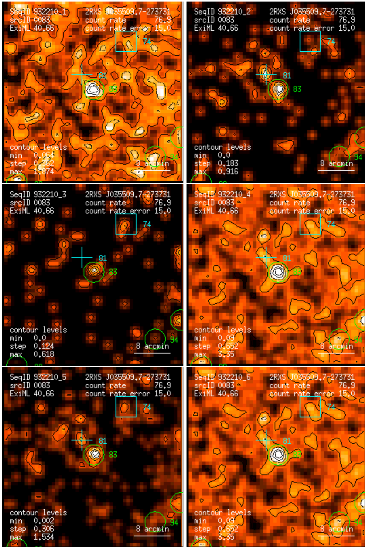
Figure 83: RASS 932210: detection 0083: band rate images, Gaussian filter: (1) PSPC channels 11 – 41, (2) 52 – 90, (3) 91 – 201, (4) 11 – 235, (5) 52 – 201, (6) 11 – 201. Broad band rates in counts/ks. Band rate contour levels in counts/ks/arcmin 2 .
