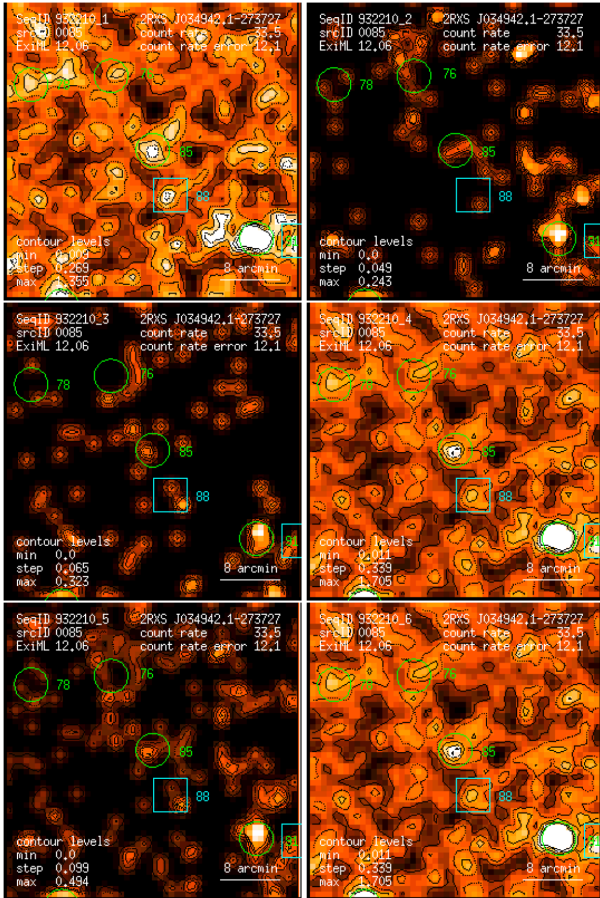
Figure 85: RASS 932210: detection 0085: band rate images, Gaussian filter: (1) PSPC channels 11 – 41, (2) 52 – 90, (3) 91 – 201, (4) 11 – 235, (5) 52 – 201, (6) 11 – 201. Broad band rates in counts/ks. Band rate contour levels in counts/ks/arcmin 2 .
