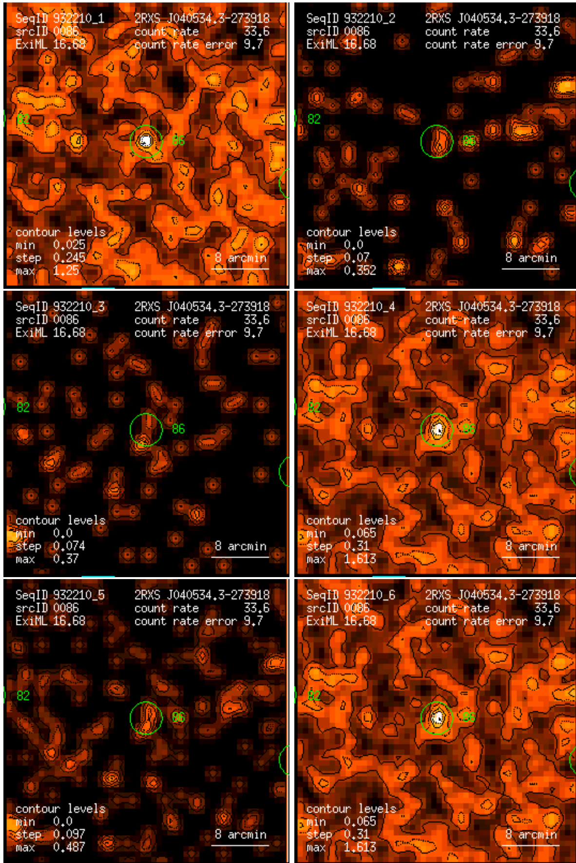
Figure 86: RASS 932210: detection 0086: band rate images, Gaussian filter: (1) PSPC channels 11 – 41, (2) 52 – 90, (3) 91 – 201, (4) 11 – 235, (5) 52 – 201, (6) 11 – 201. Broad band rates in counts/ks. Band rate contour levels in counts/ks/arcmin 2 .
