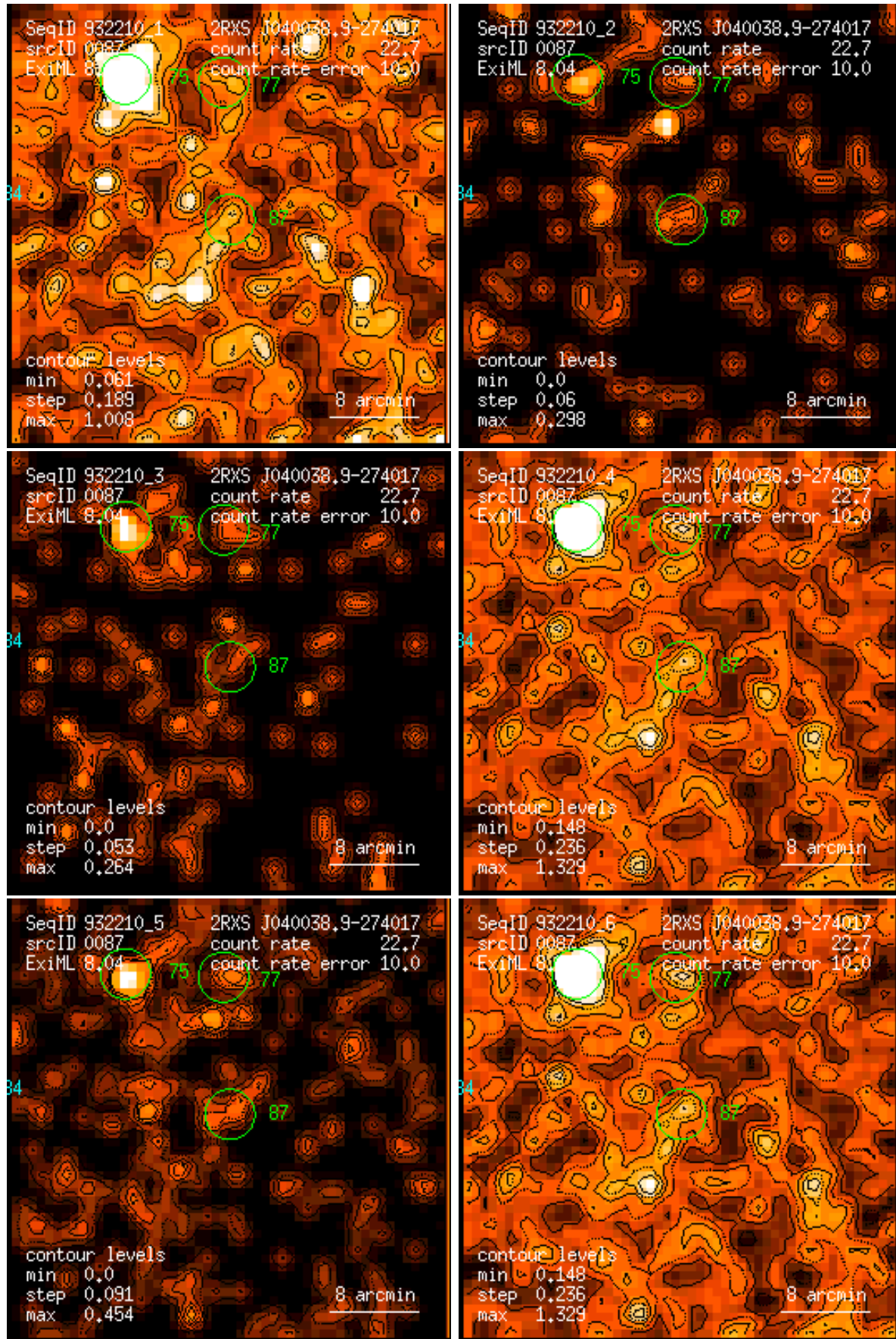
Figure 87: RASS 932210: detection 0087: band rate images, Gaussian filter: (1) PSPC channels 11 – 41, (2) 52 – 90, (3) 91 – 201, (4) 11 – 235, (5) 52 – 201, (6) 11 – 201. Broad band rates in counts/ks. Band rate contour levels in counts/ks/arcmin 2 .
