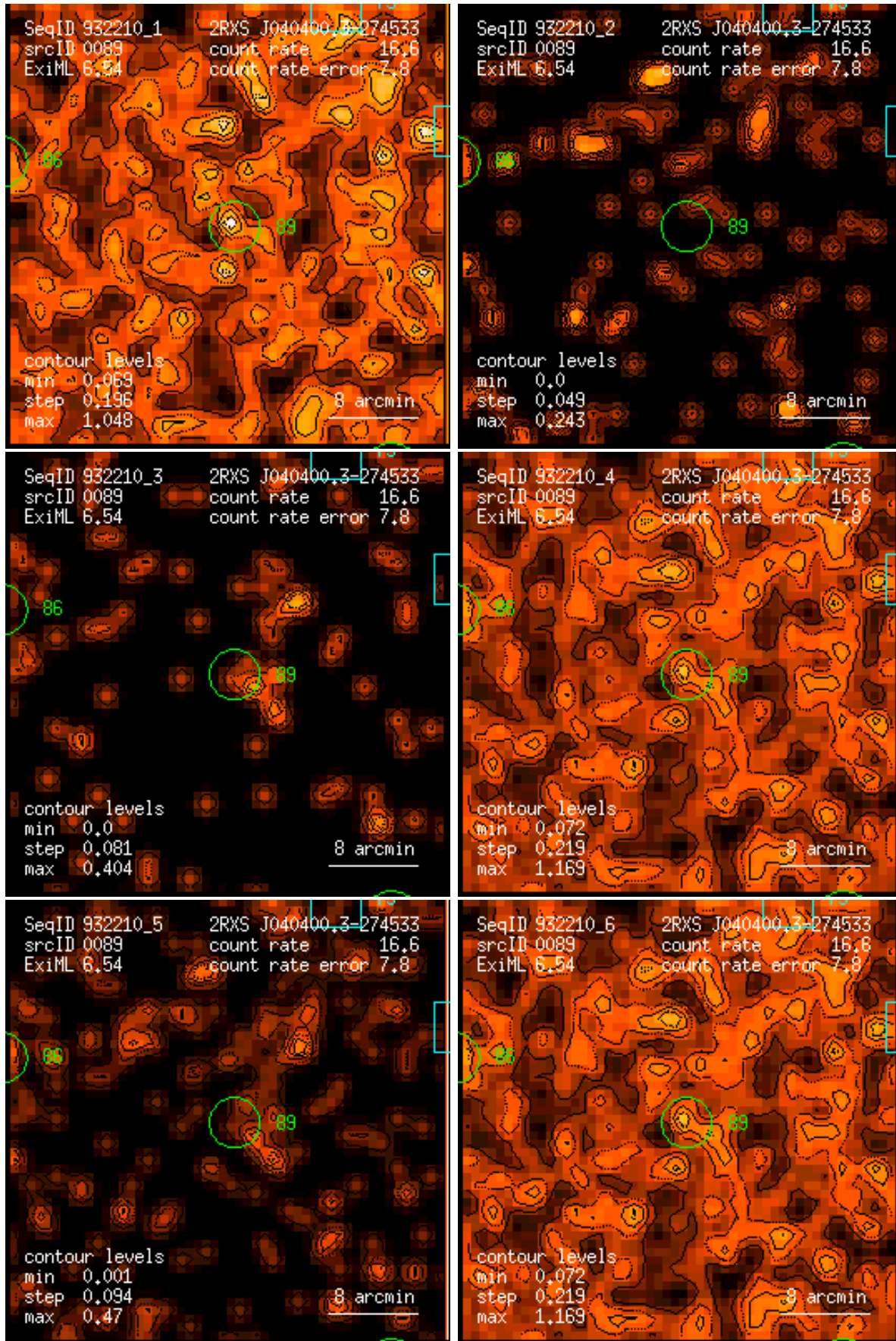
Figure 89: RASS 932210: detection 0089: band rate images, Gaussian filter: (1) PSPC channels 11 – 41, (2) 52 – 90, (3) 91 – 201, (4) 11 – 235, (5) 52 – 201, (6) 11 – 201. Broad band rates in counts/ks. Band rate contour levels in counts/ks/arcmin 2 .
