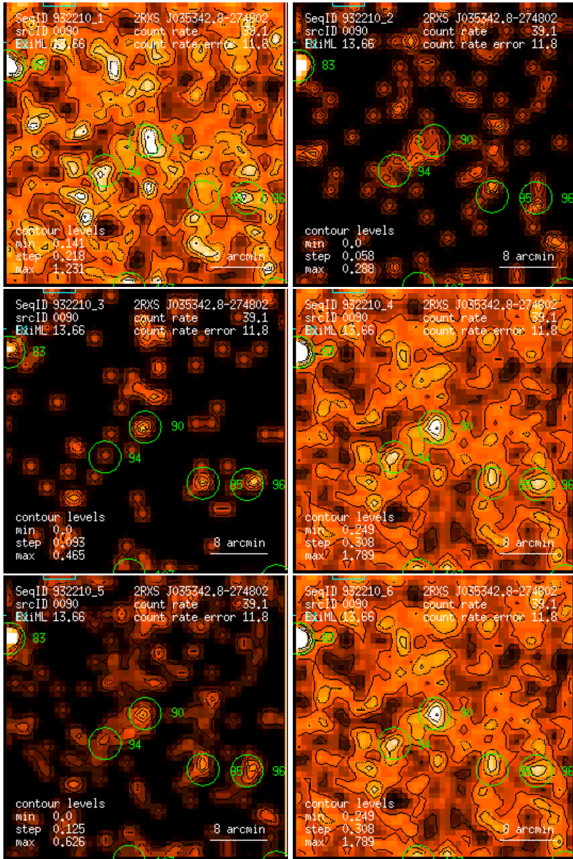
Figure 90: RASS 932210: detection 0090: band rate images, Gaussian filter: (1) PSPC channels 11 – 41, (2) 52 – 90, (3) 91 – 201, (4) 11 – 235, (5) 52 – 201, (6) 11 – 201. Broad band rates in counts/ks. Band rate contour levels in counts/ks/arcmin 2 .
