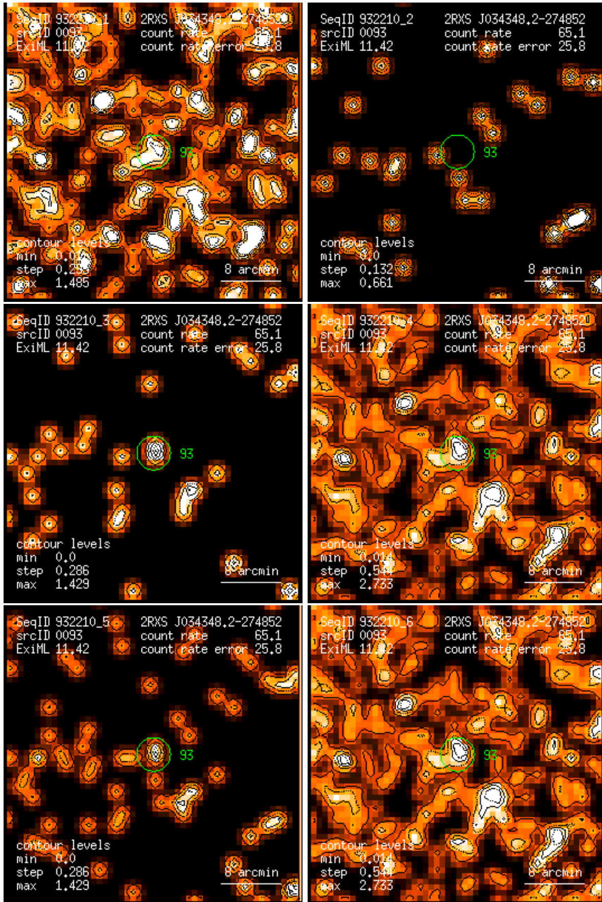
Figure 93: RASS 932210: detection 0093: band rate images, Gaussian filter: (1) PSPC channels 11 – 41, (2) 52 – 90, (3) 91 – 201, (4) 11 – 235, (5) 52 – 201, (6) 11 – 201. Broad band rates in counts/ks. Band rate contour levels in counts/ks/arcmin 2 .
