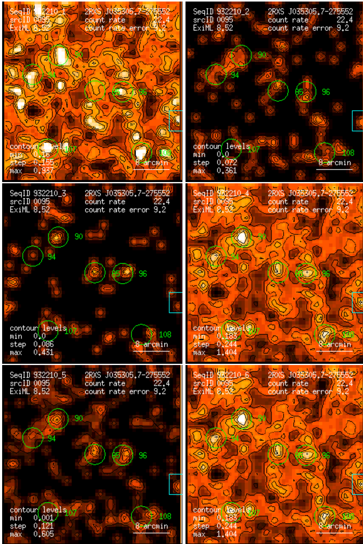
Figure 95: RASS 932210: detection 0095: band rate images, Gaussian filter: (1) PSPC channels 11 – 41, (2) 52 – 90, (3) 91 – 201, (4) 11 – 235, (5) 52 – 201, (6) 11 – 201. Broad band rates in counts/ks. Band rate contour levels in counts/ks/arcmin 2 .
