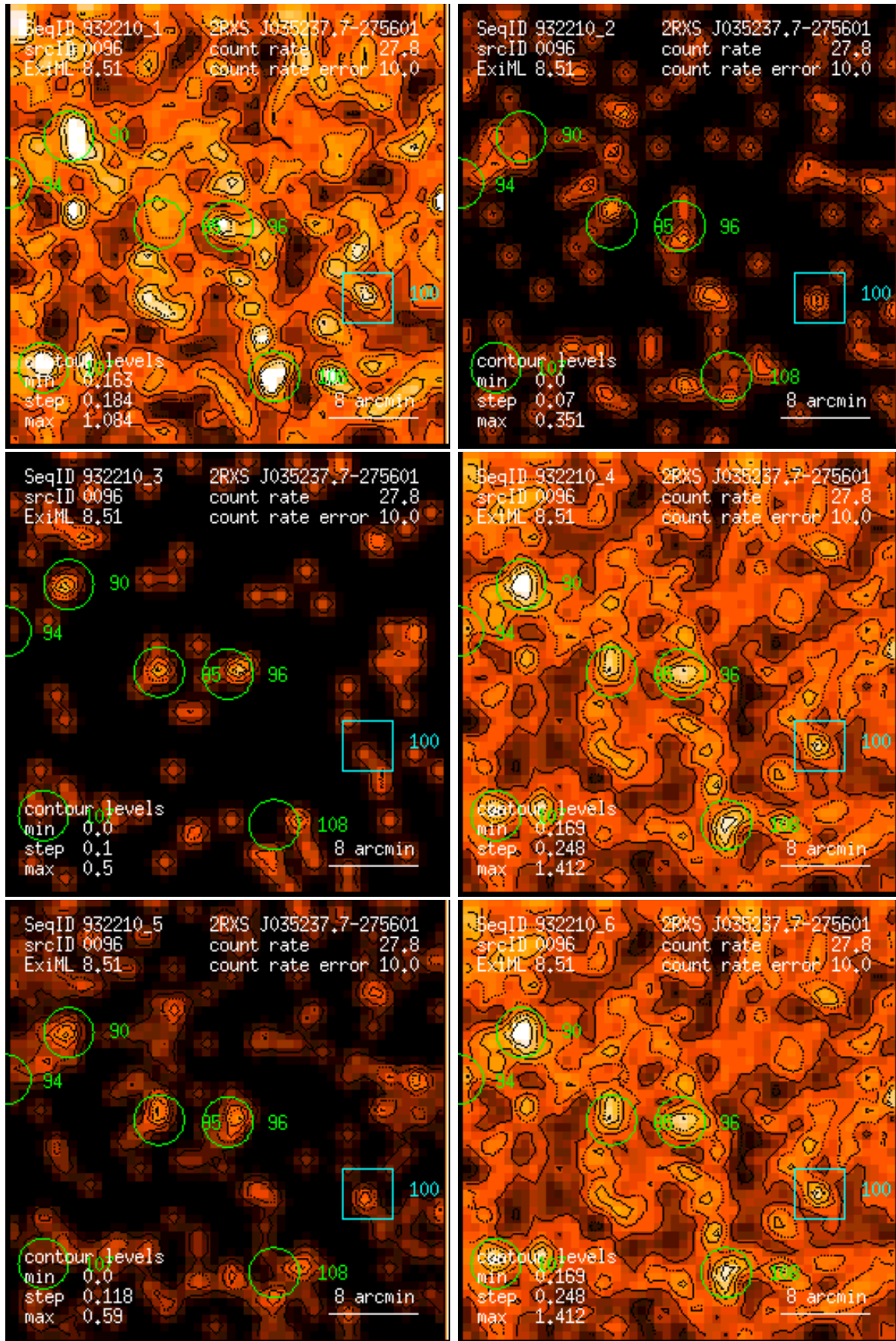
Figure 96: RASS 932210: detection 0096: band rate images, Gaussian filter: (1) PSPC channels 11 – 41, (2) 52 – 90, (3) 91 – 201, (4) 11 – 235, (5) 52 – 201, (6) 11 – 201. Broad band rates in counts/ks. Band rate contour levels in counts/ks/arcmin 2 .
