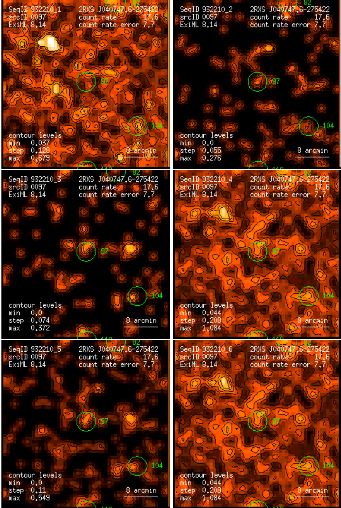
Figure 97: RASS 932210: detection 0097: band rate images, Gaussian filter: (1) PSPC channels 11 – 41, (2) 52 – 90, (3) 91 – 201, (4) 11 – 235, (5) 52 – 201, (6) 11 – 201. Broad band rates in counts/ks. Band rate contour levels in counts/ks/arcmin 2 .
