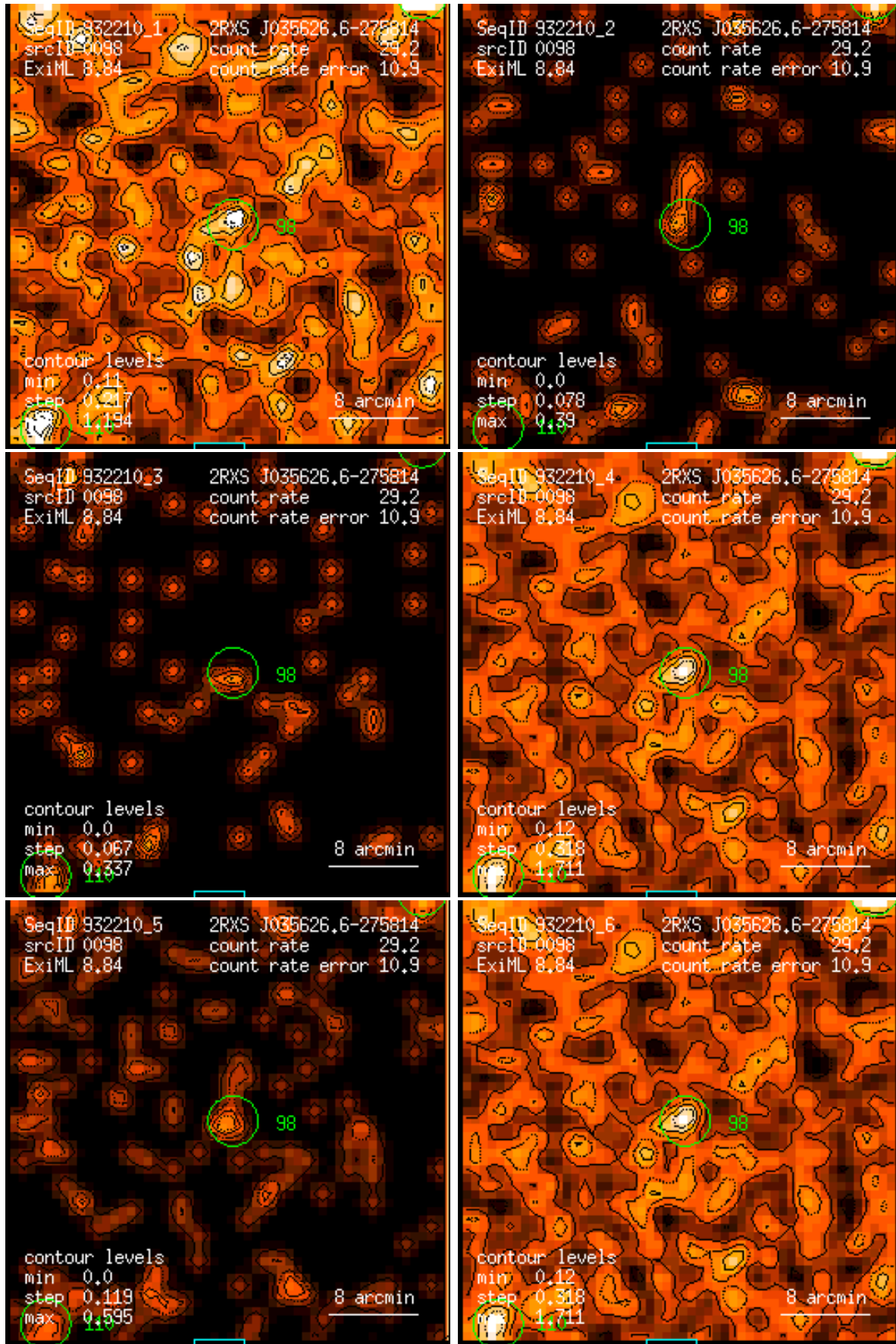
Figure 98: RASS 932210: detection 0098: band rate images, Gaussian filter: (1) PSPC channels 11 – 41, (2) 52 – 90, (3) 91 – 201, (4) 11 – 235, (5) 52 – 201, (6) 11 – 201. Broad band rates in counts/ks. Band rate contour levels in counts/ks/arcmin 2 .
