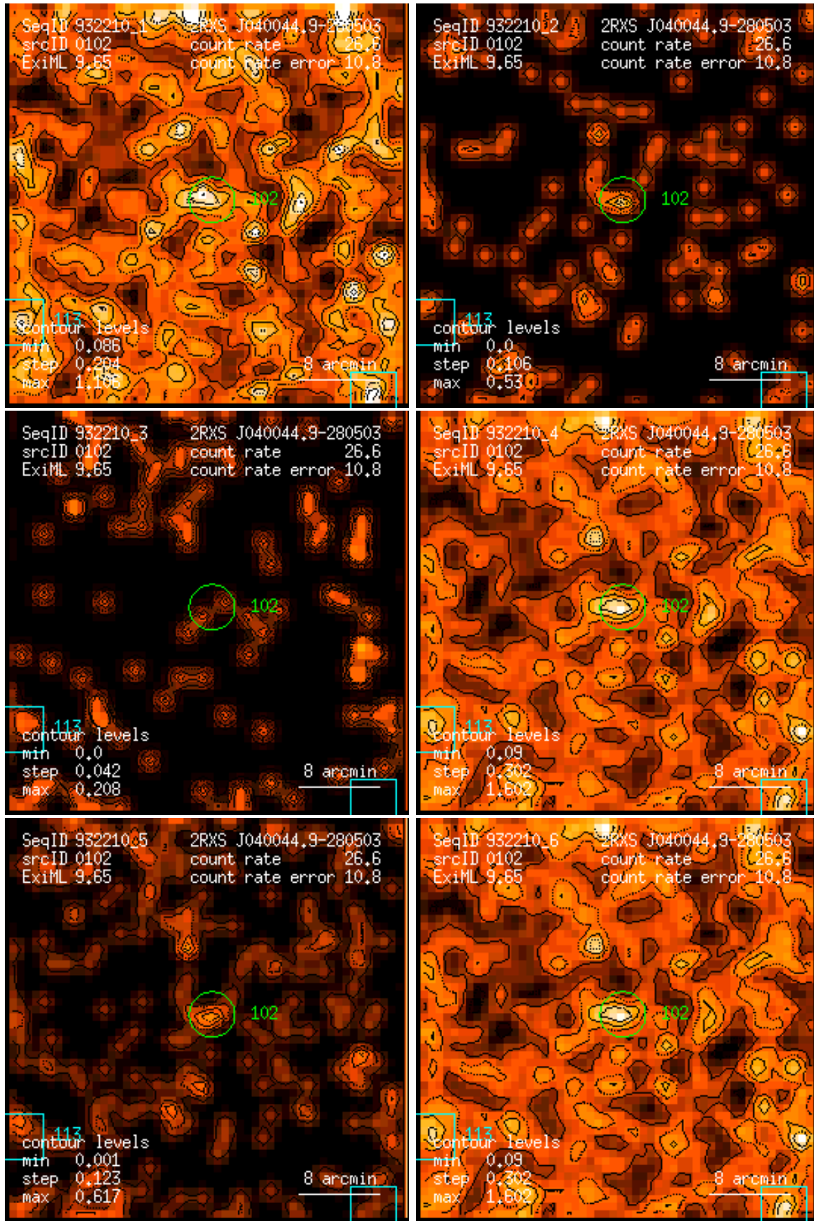
Figure 102: RASS 932210: detection 0102: band rate images, Gaussian filter: (1) PSPC channels 11 – 41, (2) 52 – 90, (3) 91 – 201, (4) 11 – 235, (5) 52 – 201, (6) 11 – 201. Broad band rates in counts/ks. Band rate contour levels in counts/ks/arcmin 2 .
