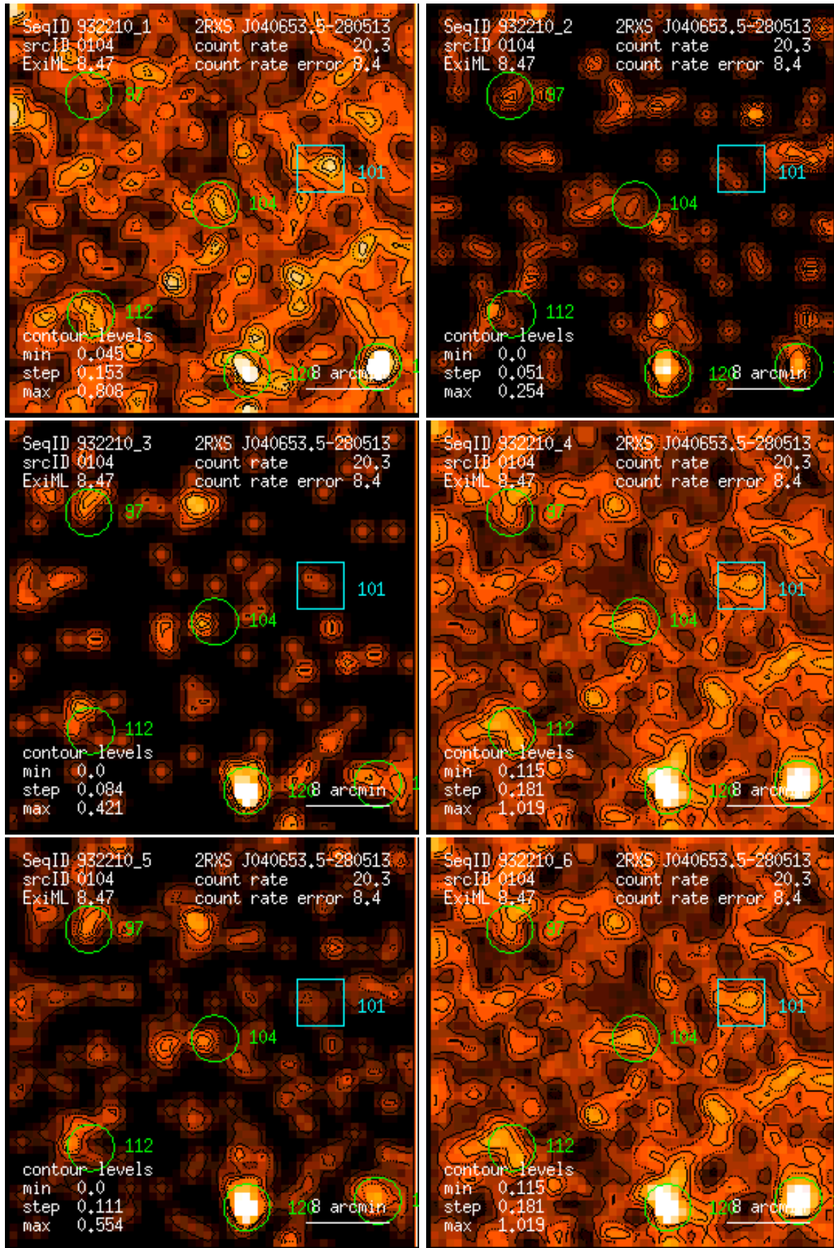
Figure 104: RASS 932210: detection 0104: band rate images, Gaussian filter: (1) PSPC channels 11 – 41, (2) 52 – 90, (3) 91 – 201, (4) 11 – 235, (5) 52 – 201, (6) 11 – 201. Broad band rates in counts/ks. Band rate contour levels in counts/ks/arcmin 2 .
